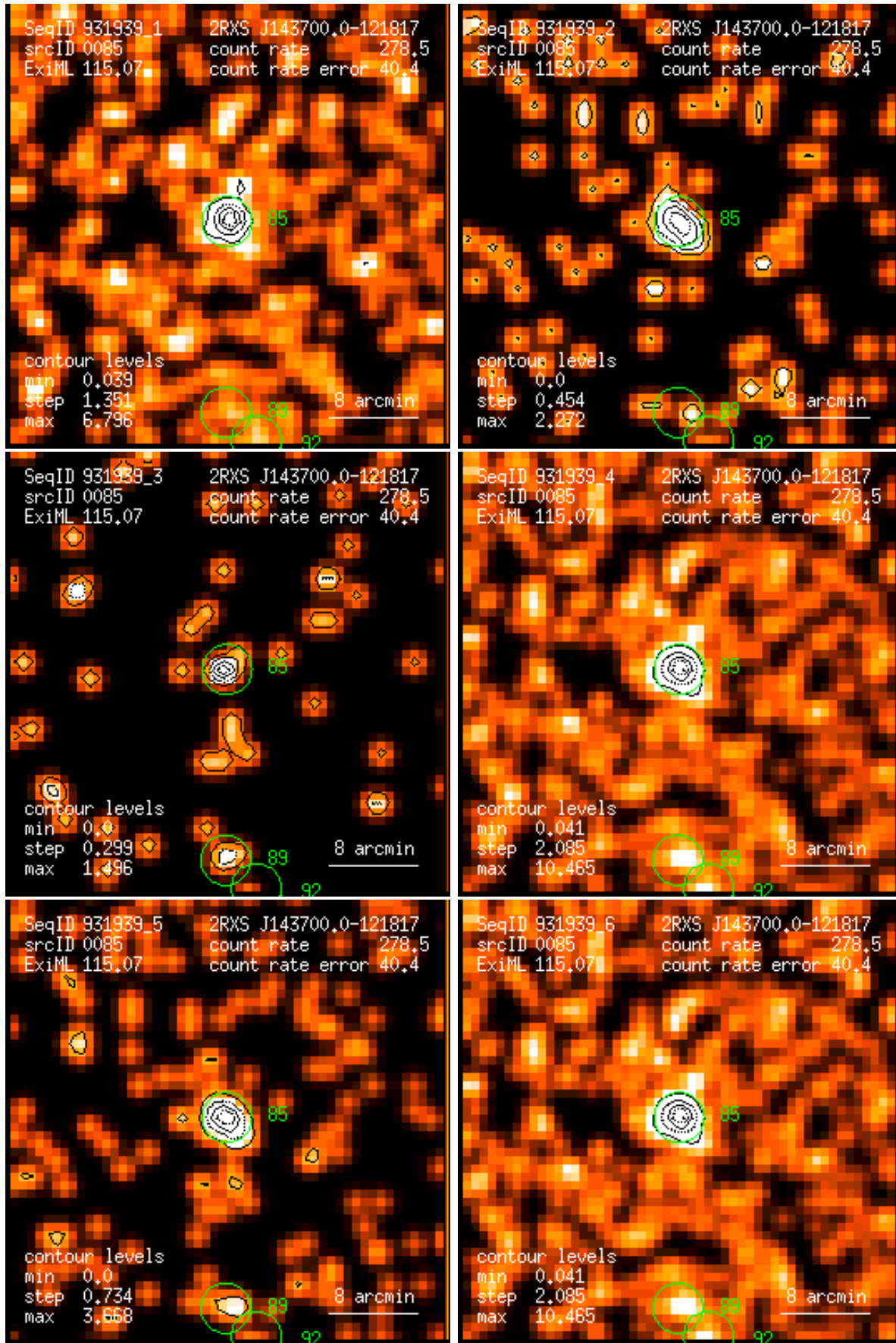
Figure 85: RASS 931939: detection 0085: band rate images, Gaussian filter: (1) PSPC channels 11 – 41, (2) 52 – 90, (3) 91 – 201, (4) 11 – 235, (5) 52 – 201, (6) 11 – 201. Broad band rates in counts/ks. Band rate contour levels in counts/ks/arcmin 2 .
