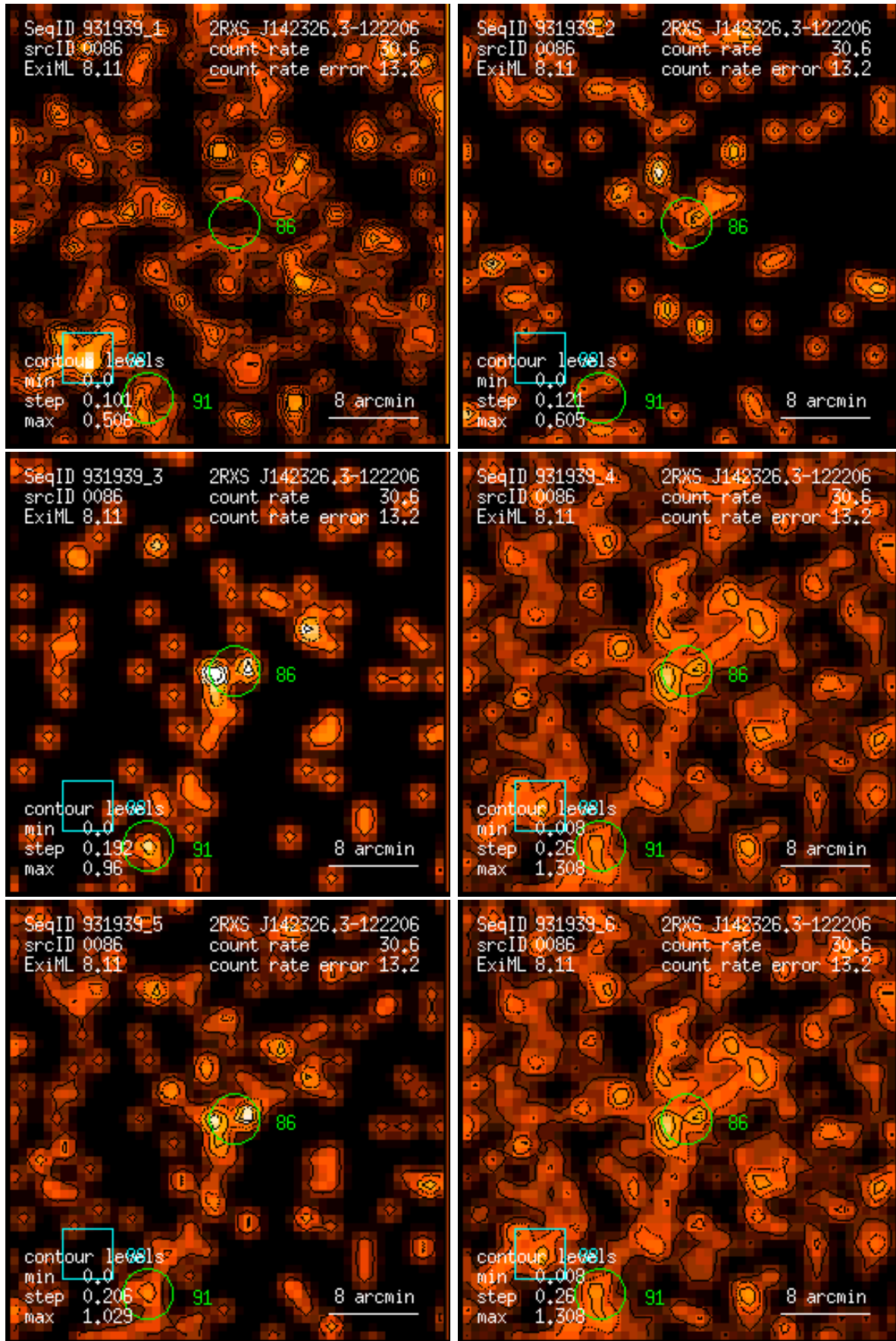
Figure 86: RASS 931939: detection 0086: band rate images, Gaussian filter: (1) PSPC channels 11 – 41, (2) 52 – 90, (3) 91 – 201, (4) 11 – 235, (5) 52 – 201, (6) 11 – 201. Broad band rates in counts/ks. Band rate contour levels in counts/ks/arcmin 2 .
