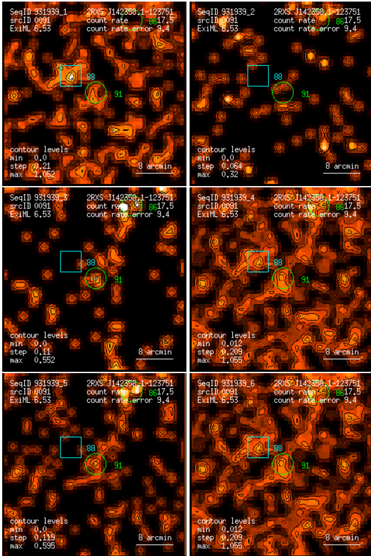
Figure 91: RASS 931939: detection 0091: band rate images, Gaussian filter: (1) PSPC channels 11 – 41, (2) 52 – 90, (3) 91 – 201, (4) 11 – 235, (5) 52 – 201, (6) 11 – 201. Broad band rates in counts/ks. Band rate contour levels in counts/ks/arcmin 2 .
