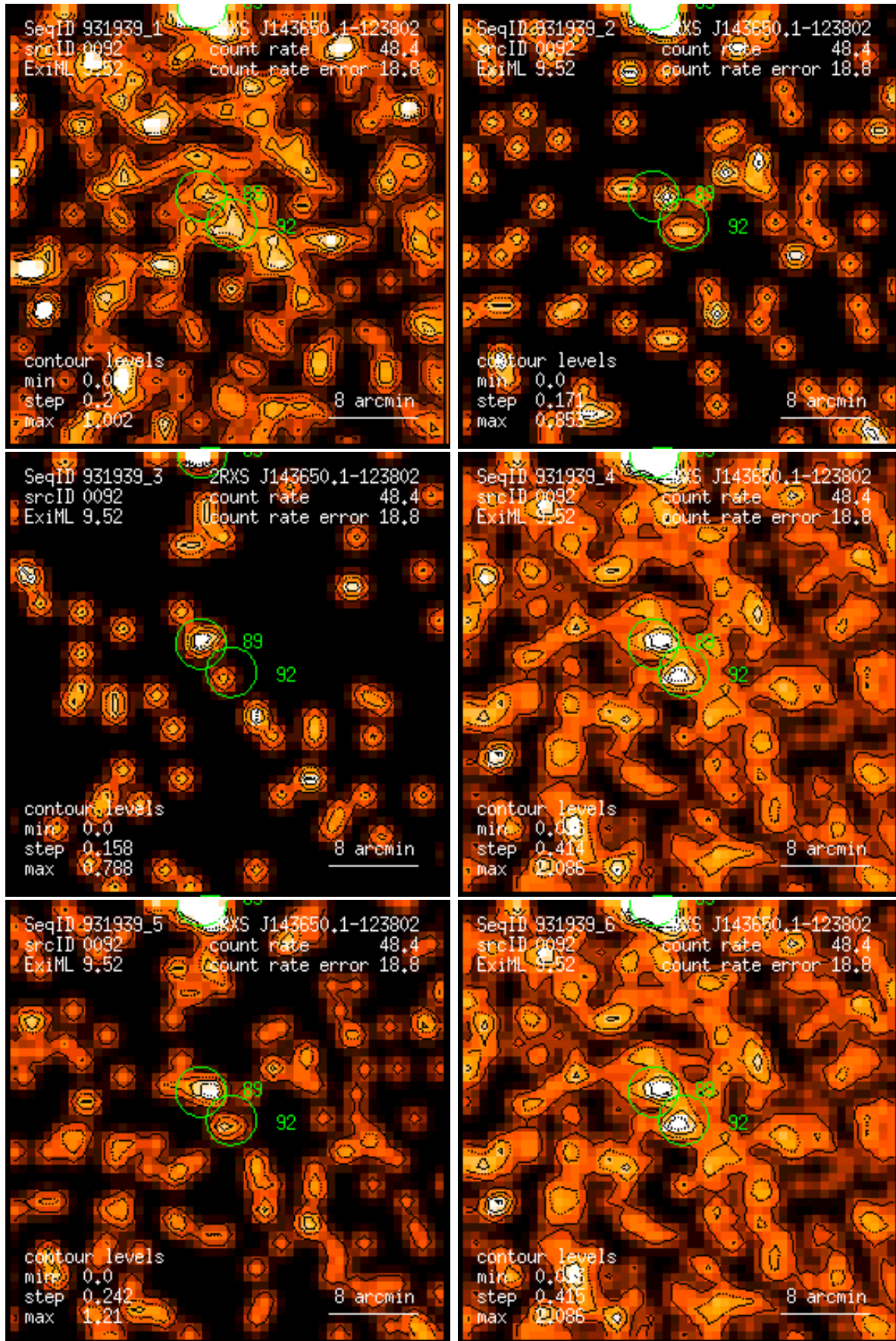
Figure 92: RASS 931939: detection 0092: band rate images, Gaussian filter: (1) PSPC channels 11 – 41, (2) 52 – 90, (3) 91 – 201, (4) 11 – 235, (5) 52 – 201, (6) 11 – 201. Broad band rates in counts/ks. Band rate contour levels in counts/ks/arcmin 2 .
