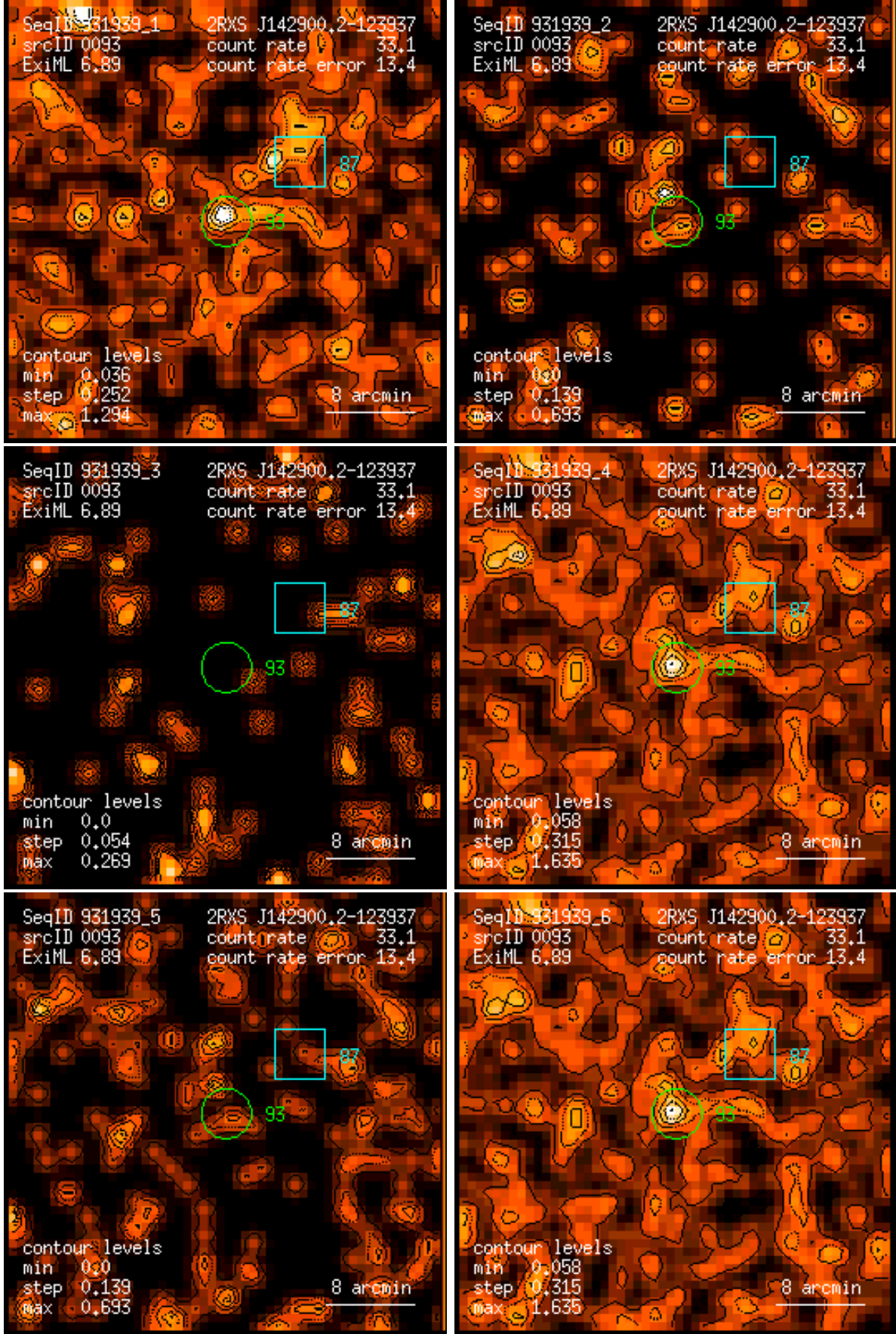
Figure 93: RASS 931939: detection 0093: band rate images, Gaussian filter: (1) PSPC channels 11 – 41, (2) 52 – 90, (3) 91 – 201, (4) 11 – 235, (5) 52 – 201, (6) 11 – 201. Broad band rates in counts/ks. Band rate contour levels in counts/ks/arcmin 2 .
