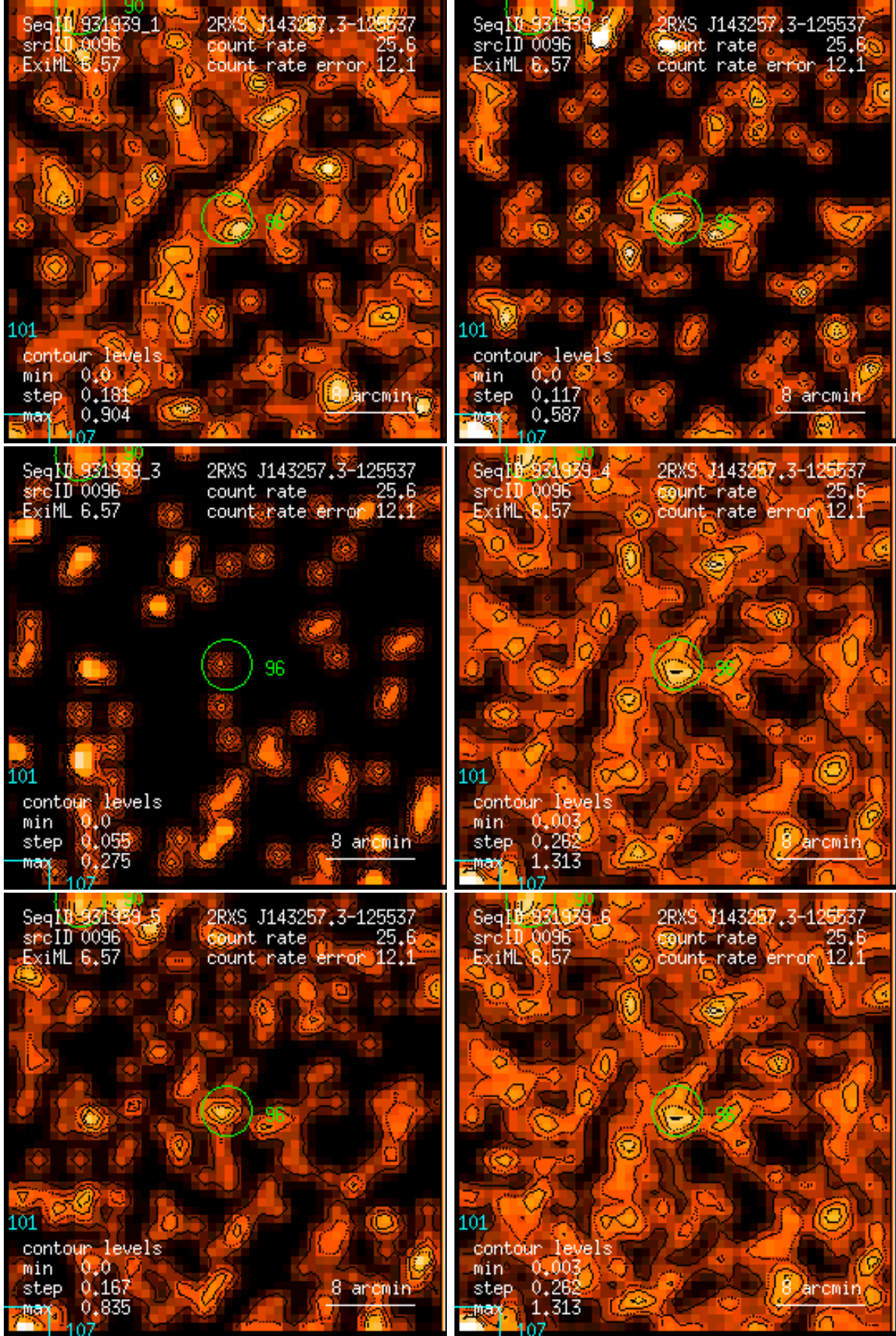
Figure 96: RASS 931939: detection 0096: band rate images, Gaussian filter: (1) PSPC channels 11 – 41, (2) 52 – 90, (3) 91 – 201, (4) 11 – 235, (5) 52 – 201, (6) 11 – 201. Broad band rates in counts/ks. Band rate contour levels in counts/ks/arcmin 2 .
