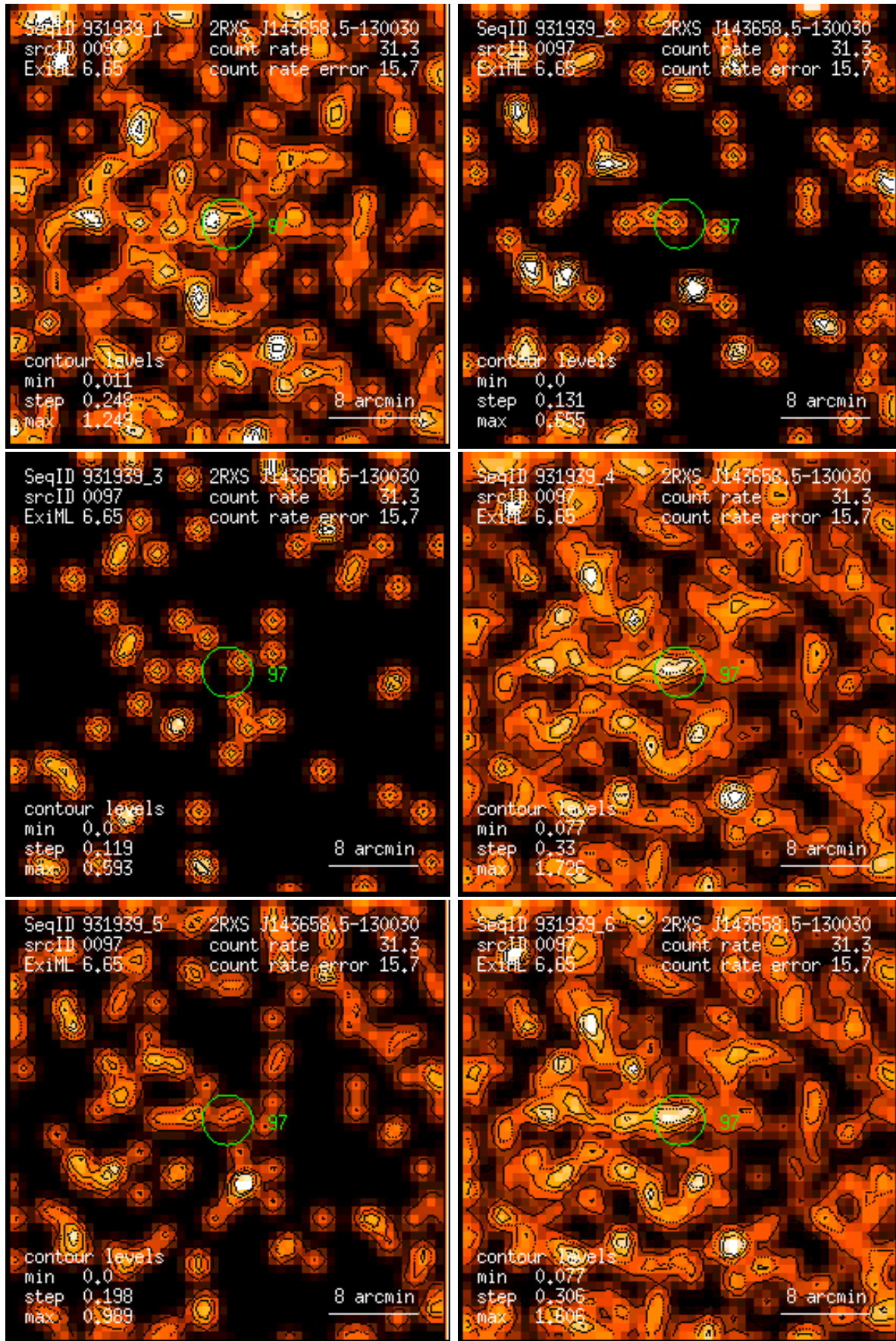
Figure 97: RASS 931939: detection 0097: band rate images, Gaussian filter: (1) PSPC channels 11 – 41, (2) 52 – 90, (3) 91 – 201, (4) 11 – 235, (5) 52 – 201, (6) 11 – 201. Broad band rates in counts/ks. Band rate contour levels in counts/ks/arcmin 2 .
