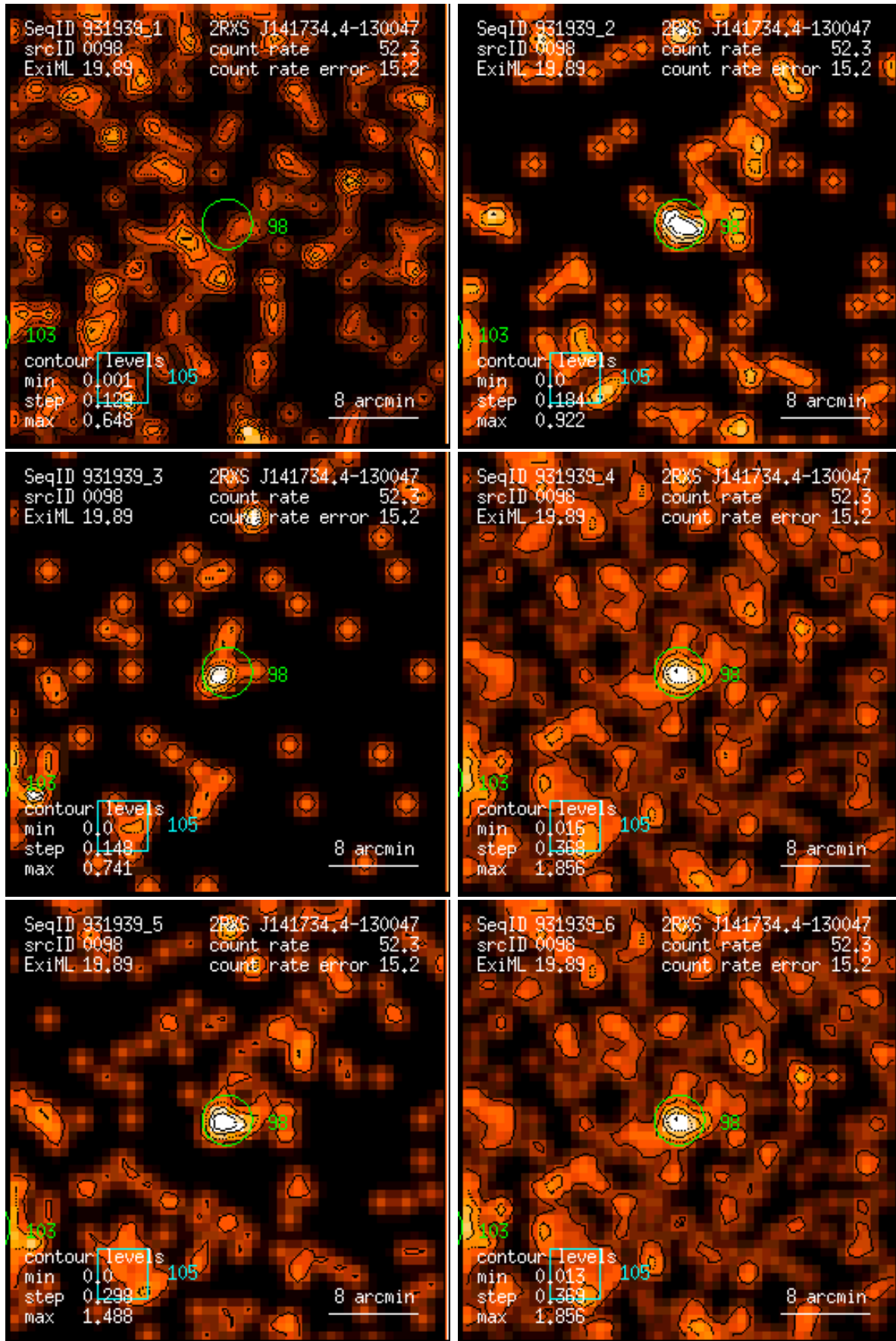
Figure 98: RASS 931939: detection 0098: band rate images, Gaussian filter: (1) PSPC channels 11 – 41, (2) 52 – 90, (3) 91 – 201, (4) 11 – 235, (5) 52 – 201, (6) 11 – 201. Broad band rates in counts/ks. Band rate contour levels in counts/ks/arcmin 2 .
