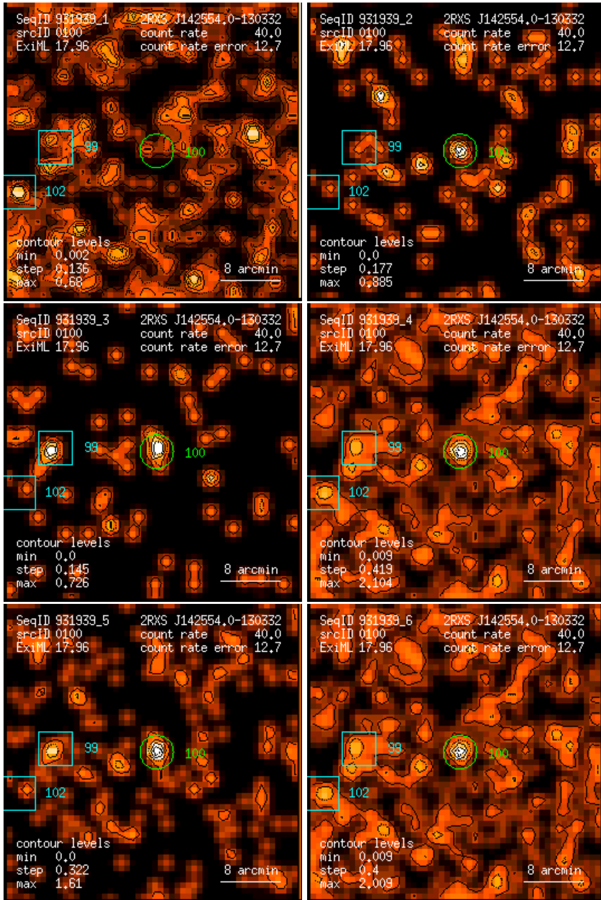
Figure 100: RASS 931939: detection 0100: band rate images, Gaussian filter: (1) PSPC channels 11 – 41, (2) 52 – 90, (3) 91 – 201, (4) 11 – 235, (5) 52 – 201, (6) 11 – 201. Broad band rates in counts/ks. Band rate contour levels in counts/ks/arcmin 2 .
