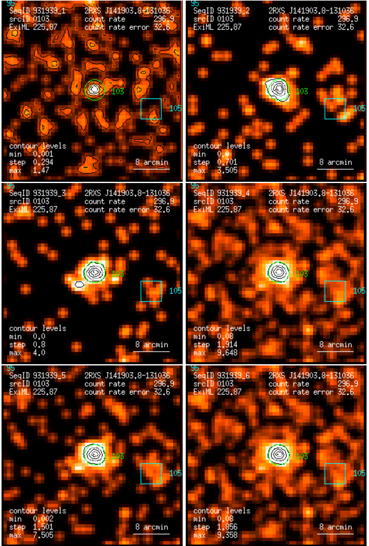
Figure 103: RASS 931939: detection 0103: band rate images, Gaussian filter: (1) PSPC channels 11 – 41, (2) 52 – 90, (3) 91 – 201, (4) 11 – 235, (5) 52 – 201, (6) 11 – 201. Broad band rates in counts/ks. Band rate contour levels in counts/ks/arcmin 2 .
