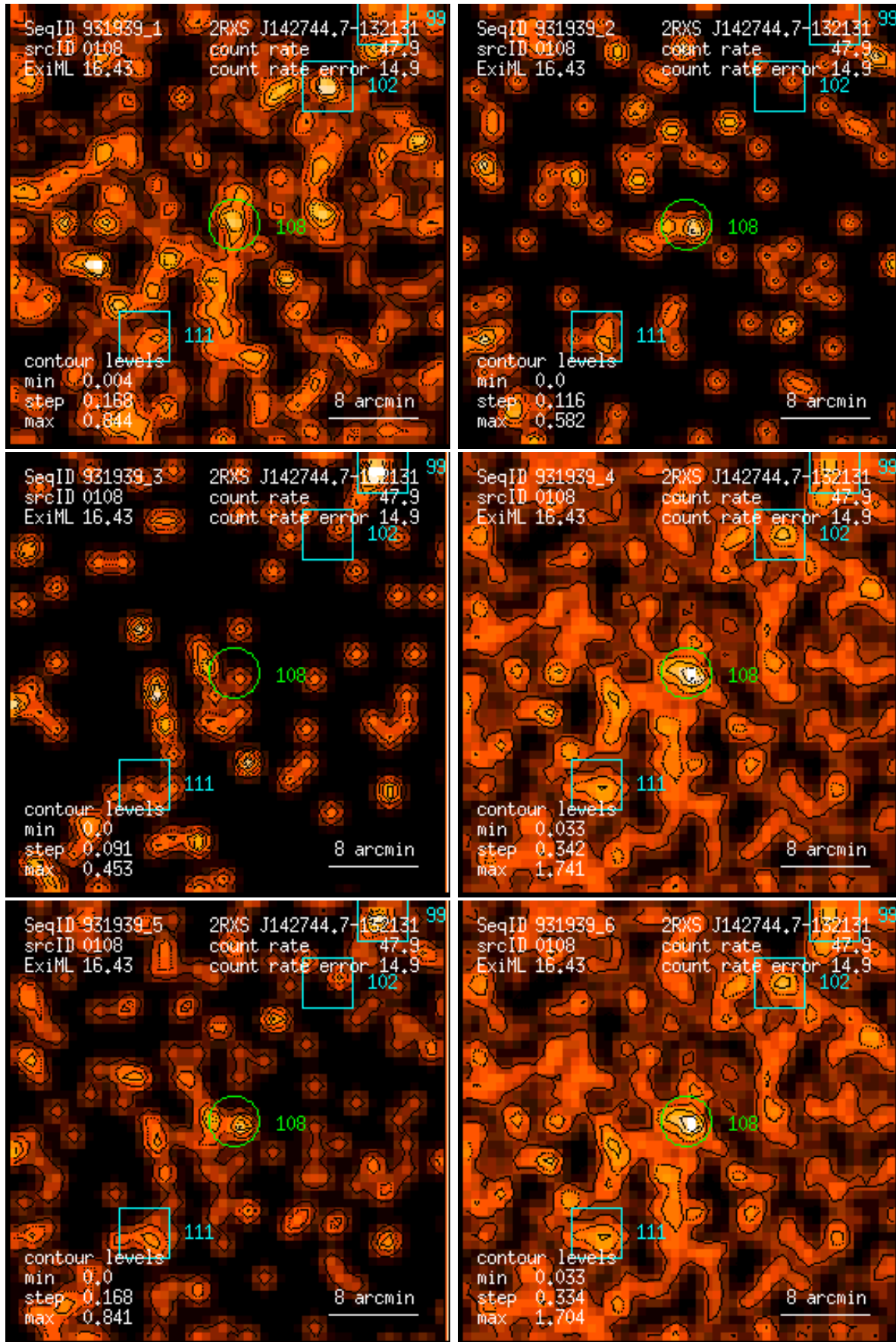
Figure 108: RASS 931939: detection 0108: band rate images, Gaussian filter: (1) PSPC channels 11 – 41, (2) 52 – 90, (3) 91 – 201, (4) 11 – 235, (5) 52 – 201, (6) 11 – 201. Broad band rates in counts/ks. Band rate contour levels in counts/ks/arcmin 2 .
