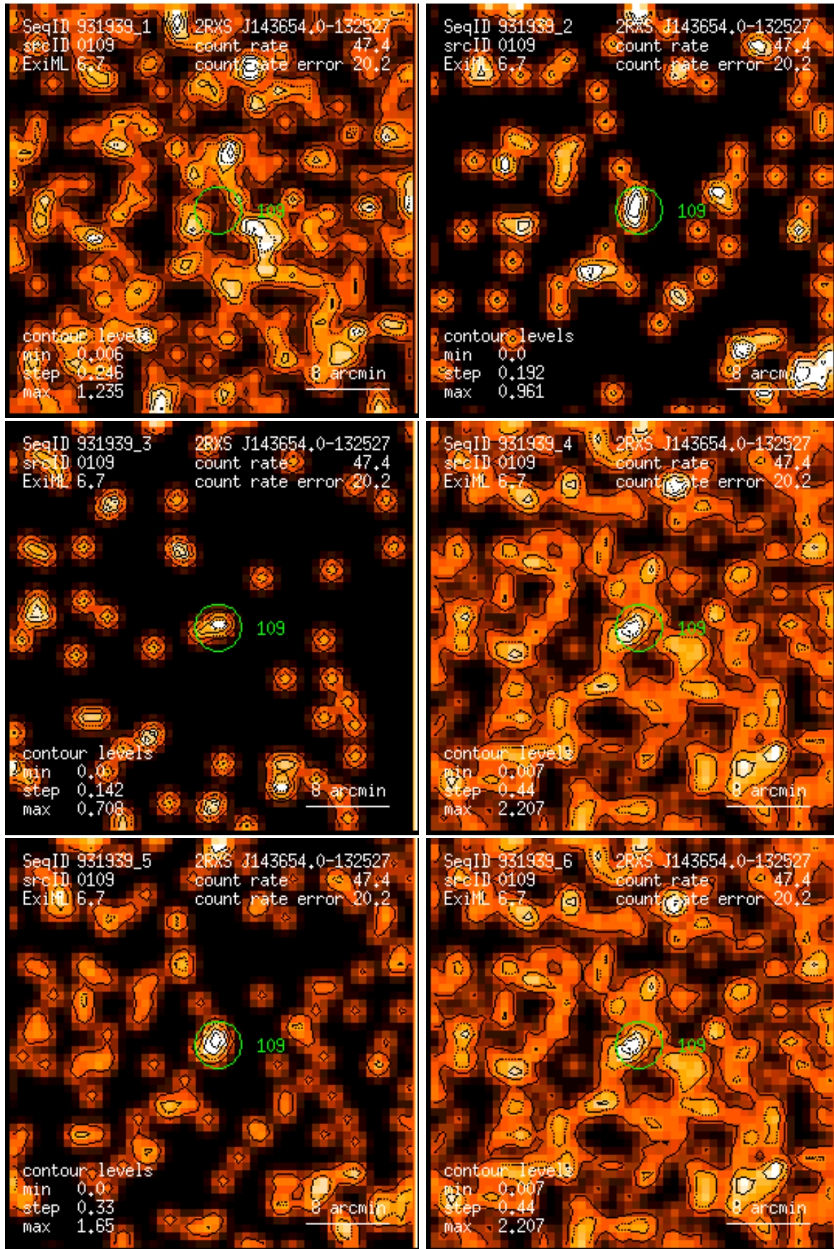
Figure 109: RASS 931939: detection 0109: band rate images, Gaussian filter: (1) PSPC channels 11 – 41, (2) 52 – 90, (3) 91 – 201, (4) 11 – 235, (5) 52 – 201, (6) 11 – 201. Broad band rates in counts/ks. Band rate contour levels in counts/ks/arcmin 2 .
