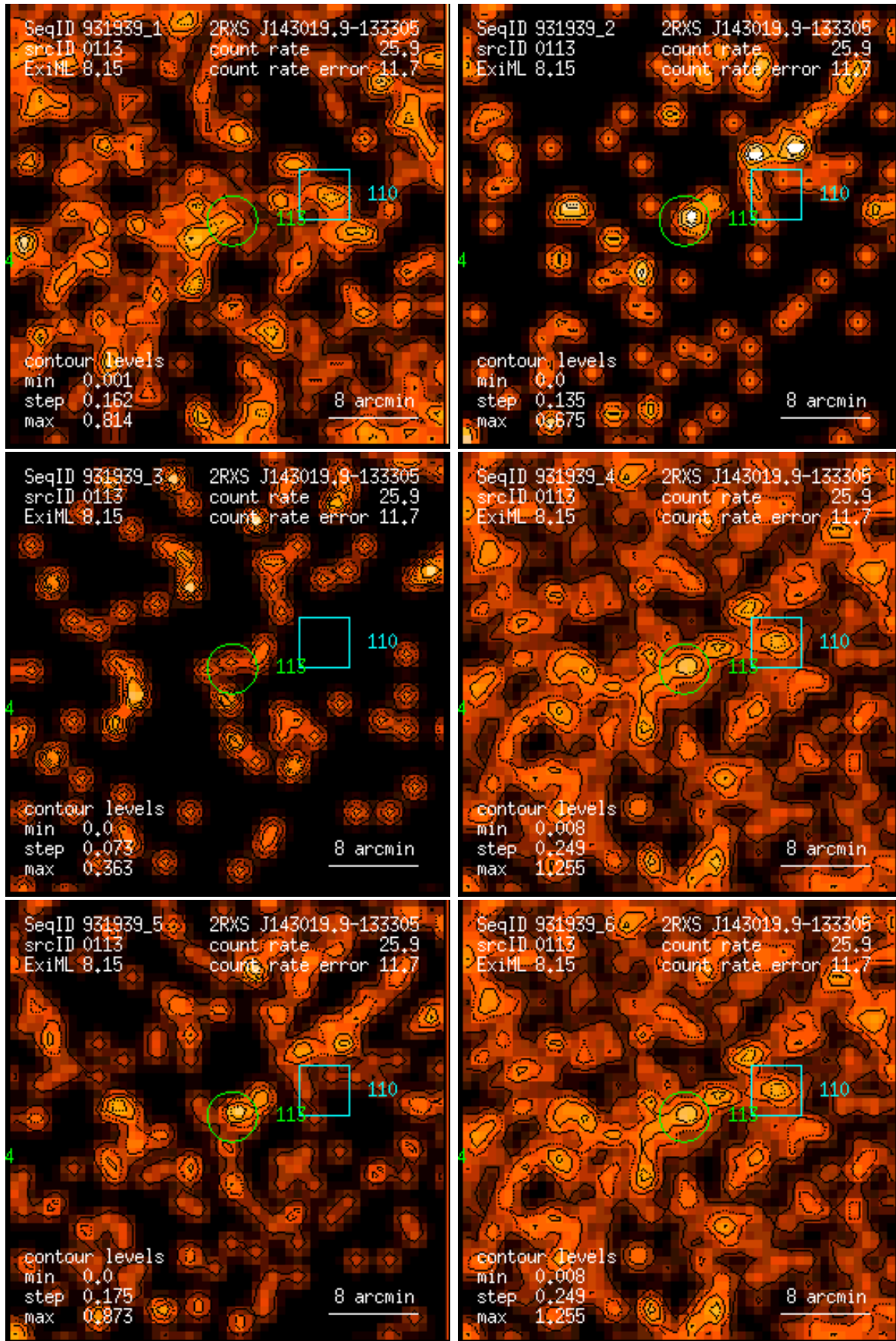
Figure 113: RASS 931939: detection 0113: band rate images, Gaussian filter: (1) PSPC channels 11 – 41, (2) 52 – 90, (3) 91 – 201, (4) 11 – 235, (5) 52 – 201, (6) 11 – 201. Broad band rates in counts/ks. Band rate contour levels in counts/ks/arcmin 2 .
