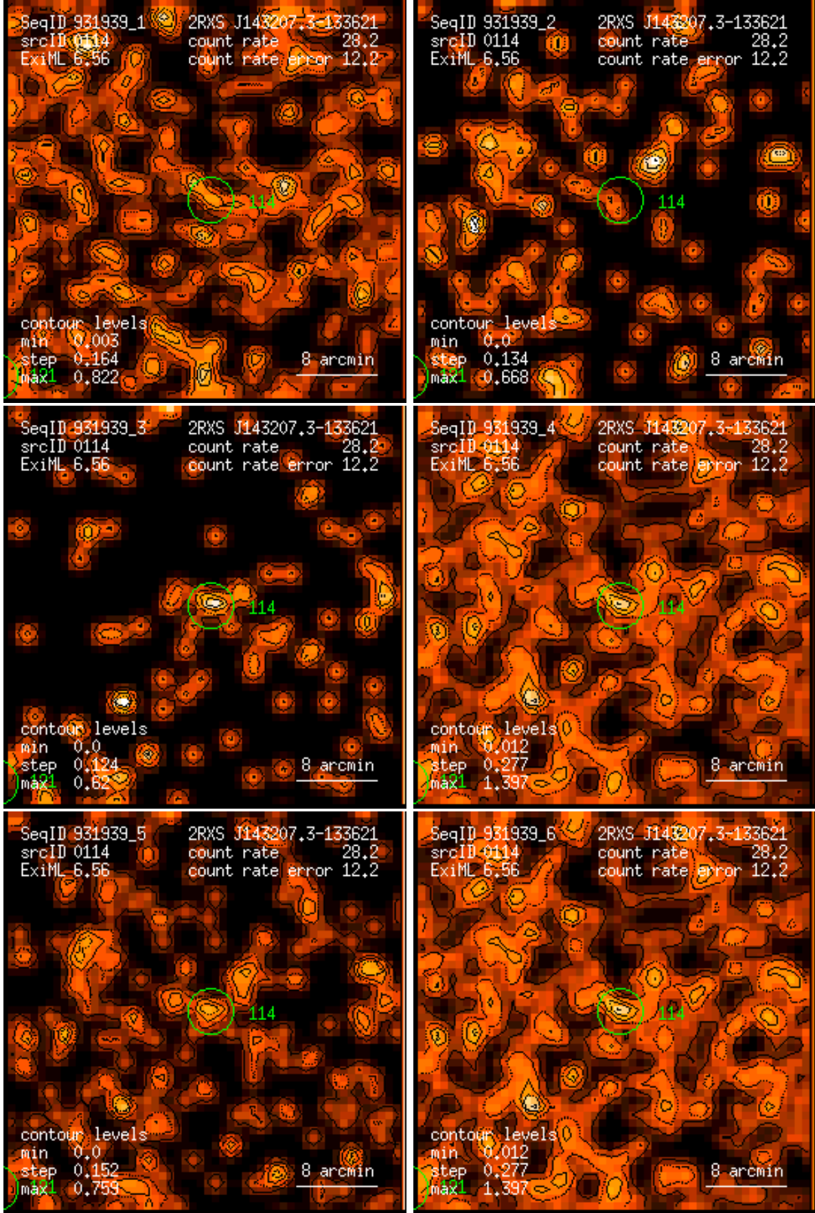
Figure 114: RASS 931939: detection 0114: band rate images, Gaussian filter: (1) PSPC channels 11 – 41, (2) 52 – 90, (3) 91 – 201, (4) 11 – 235, (5) 52 – 201, (6) 11 – 201. Broad band rates in counts/ks. Band rate contour levels in counts/ks/arcmin 2 .
