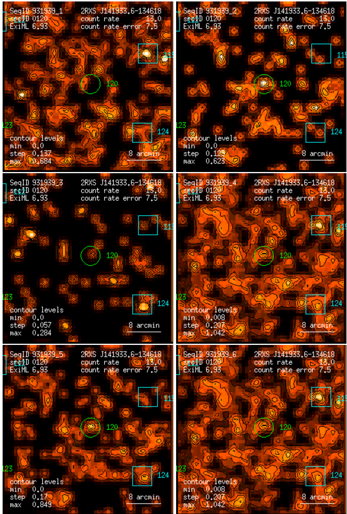
Figure 120: RASS 931939: detection 0120: band rate images, Gaussian filter: (1) PSPC channels 11 – 41, (2) 52 – 90, (3) 91 – 201, (4) 11 – 235, (5) 52 – 201, (6) 11 – 201. Broad band rates in counts/ks. Band rate contour levels in counts/ks/arcmin 2 .
