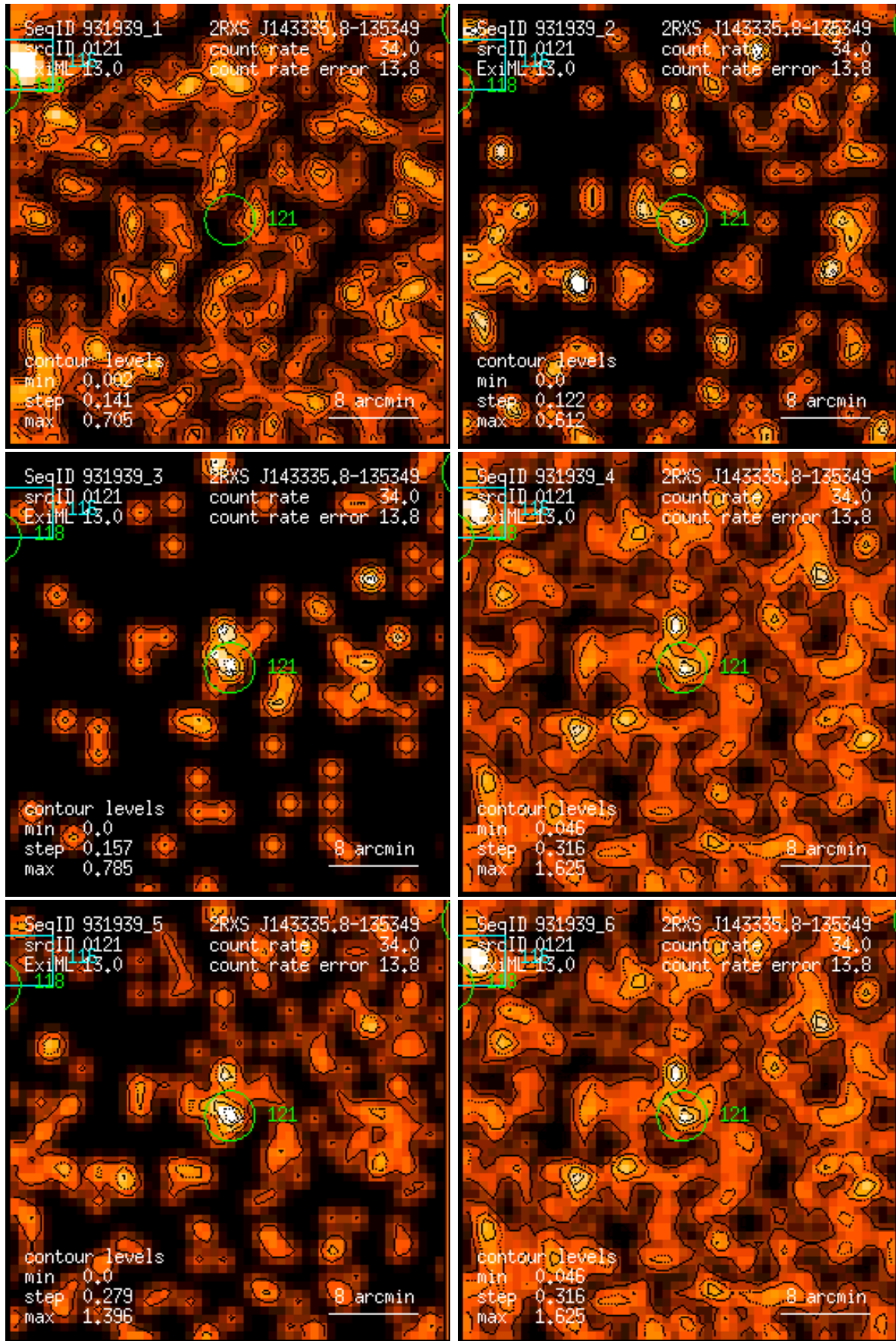
Figure 121: RASS 931939: detection 0121: band rate images, Gaussian filter: (1) PSPC channels 11 – 41, (2) 52 – 90, (3) 91 – 201, (4) 11 – 235, (5) 52 – 201, (6) 11 – 201. Broad band rates in counts/ks. Band rate contour levels in counts/ks/arcmin 2 .
