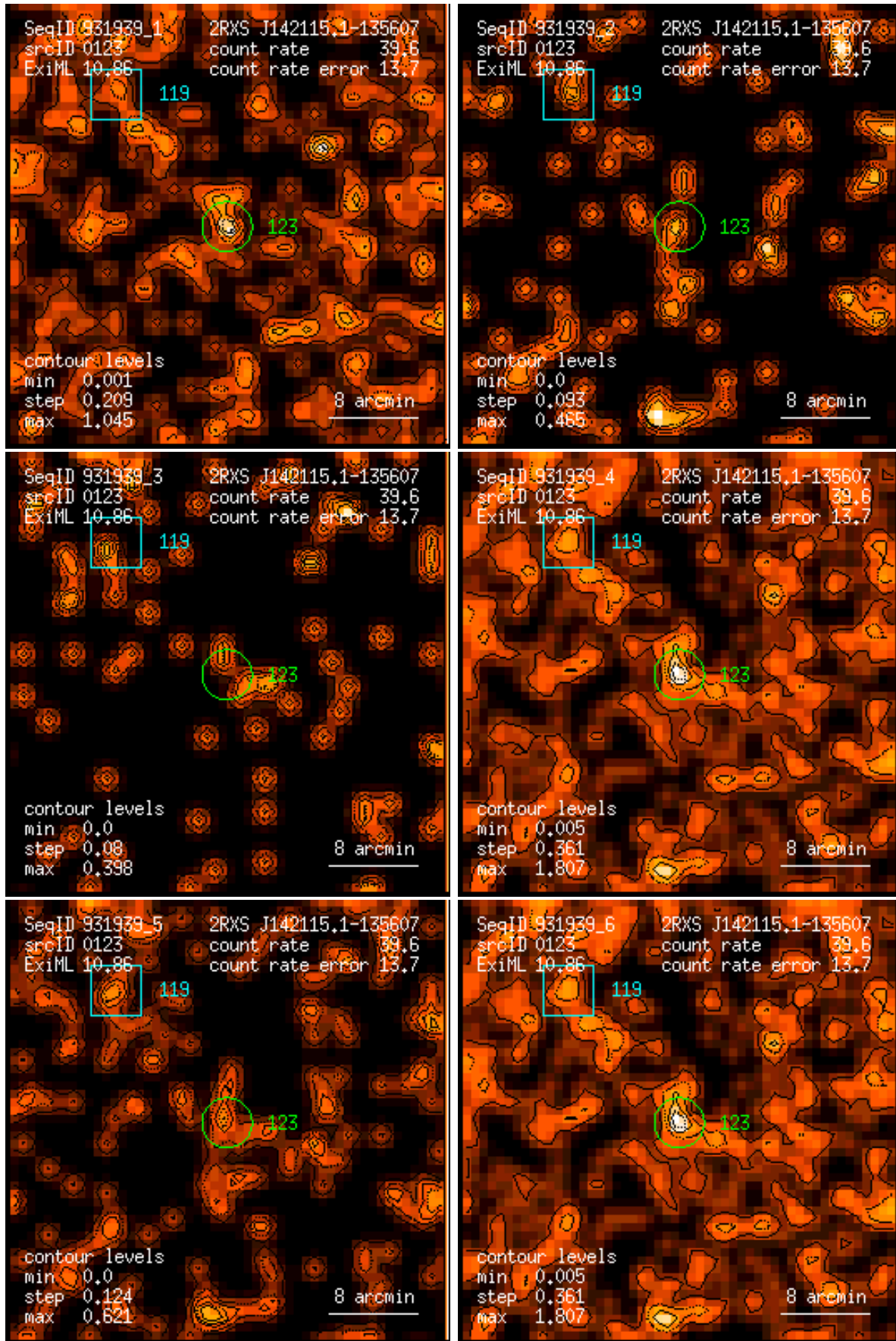
Figure 123: RASS 931939: detection 0123: band rate images, Gaussian filter: (1) PSPC channels 11 – 41, (2) 52 – 90, (3) 91 – 201, (4) 11 – 235, (5) 52 – 201, (6) 11 – 201. Broad band rates in counts/ks. Band rate contour levels in counts/ks/arcmin 2 .
