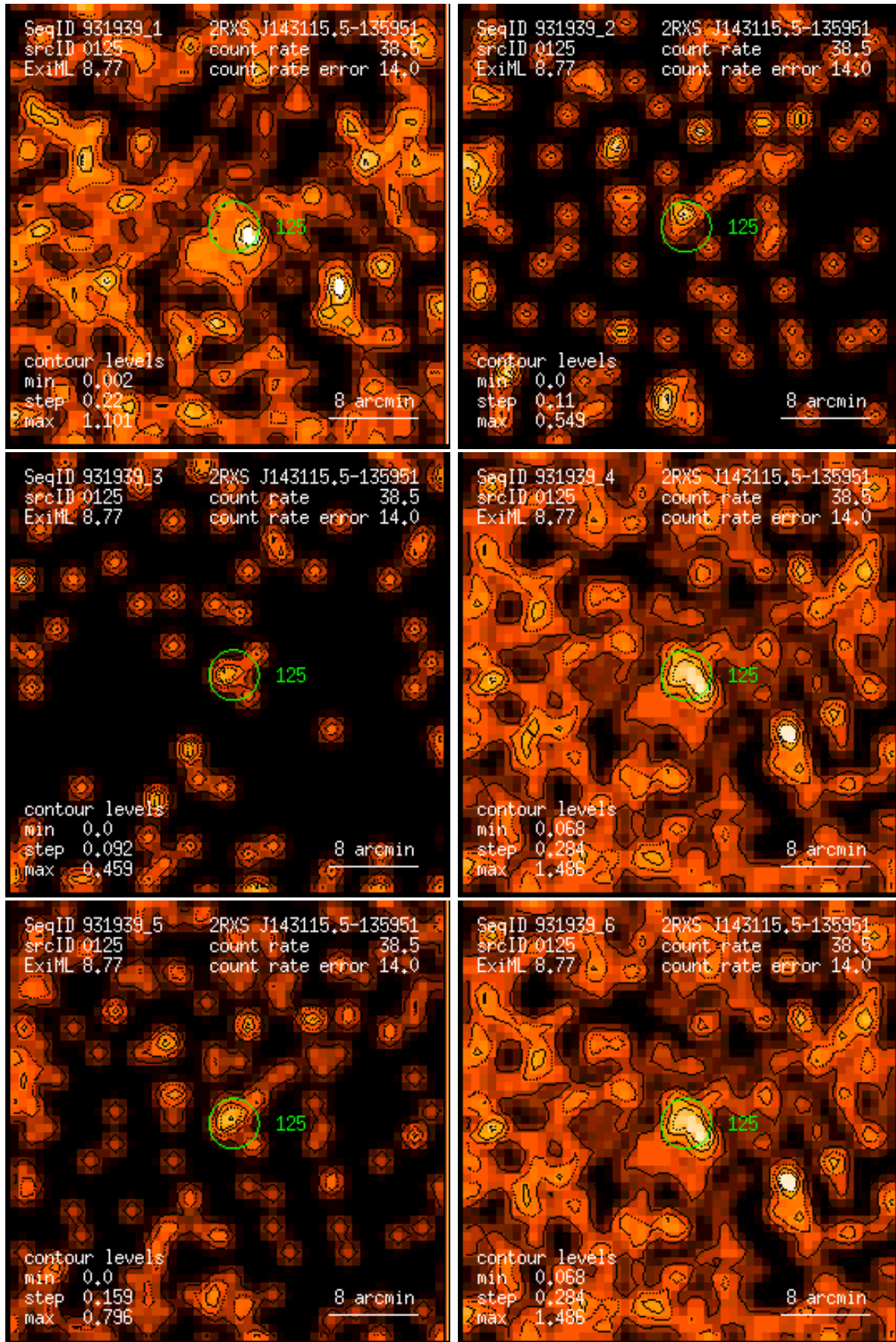
Figure 125: RASS 931939: detection 0125: band rate images, Gaussian filter: (1) PSPC channels 11 – 41, (2) 52 – 90, (3) 91 – 201, (4) 11 – 235, (5) 52 – 201, (6) 11 – 201. Broad band rates in counts/ks. Band rate contour levels in counts/ks/arcmin 2 .
