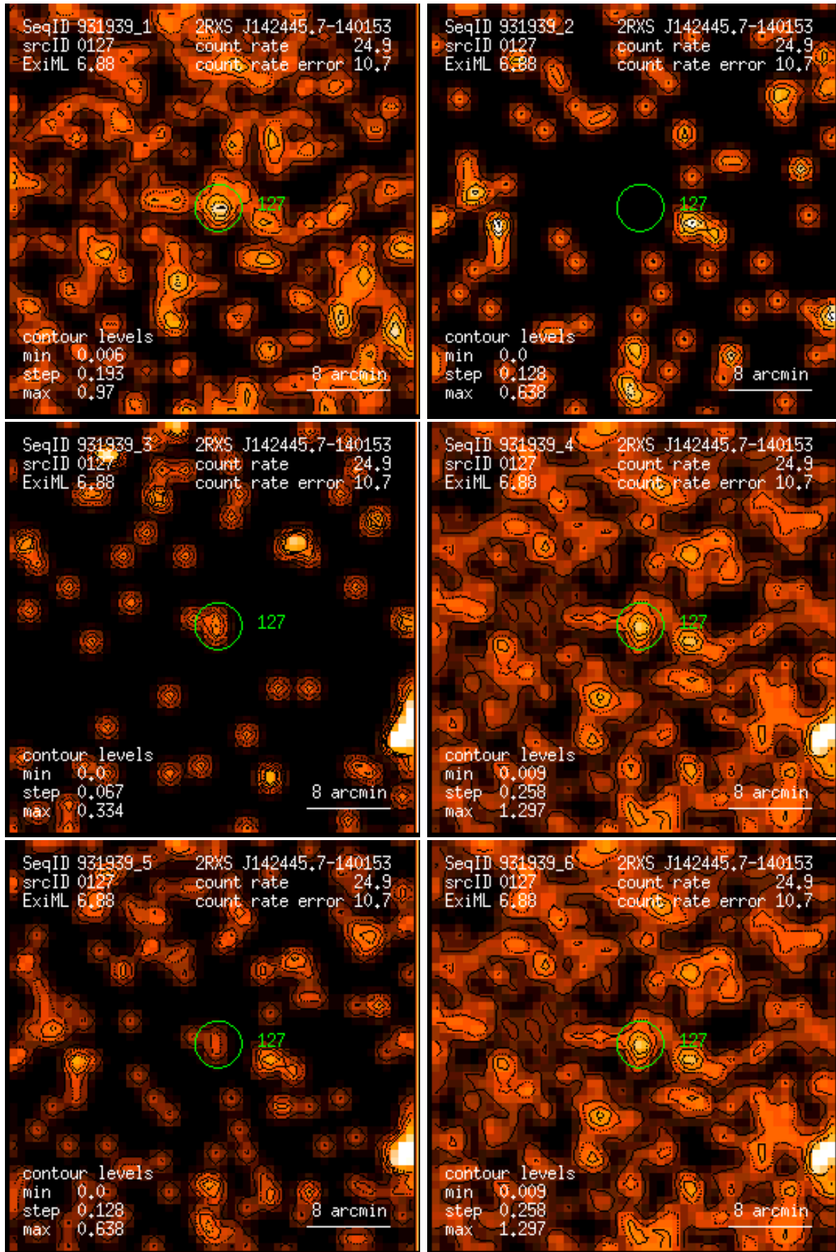
Figure 127: RASS 931939: detection 0127: band rate images, Gaussian filter: (1) PSPC channels 11 – 41, (2) 52 – 90, (3) 91 – 201, (4) 11 – 235, (5) 52 – 201, (6) 11 – 201. Broad band rates in counts/ks. Band rate contour levels in counts/ks/arcmin 2 .
