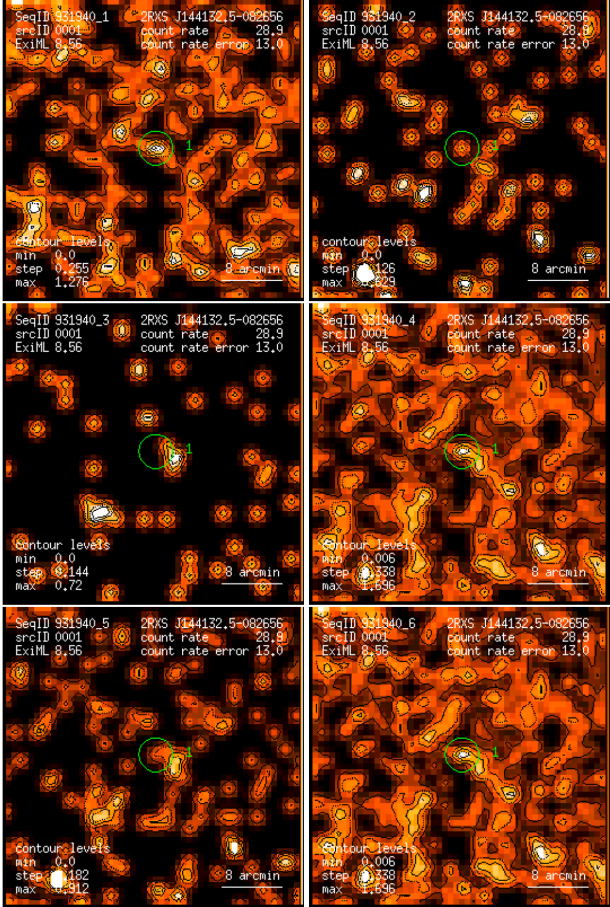
Figure 1: RASS 931940: detection 0001: band rate images, Gaussian filter: (1) PSPC channels 11 – 41, (2) 52 – 90, (3) 91 – 201, (4) 11 – 235, (5) 52 – 201, (6) 11 – 201. Broad band rates in counts/ks. Band rate contour levels in counts/ks/arcmin 2 .
