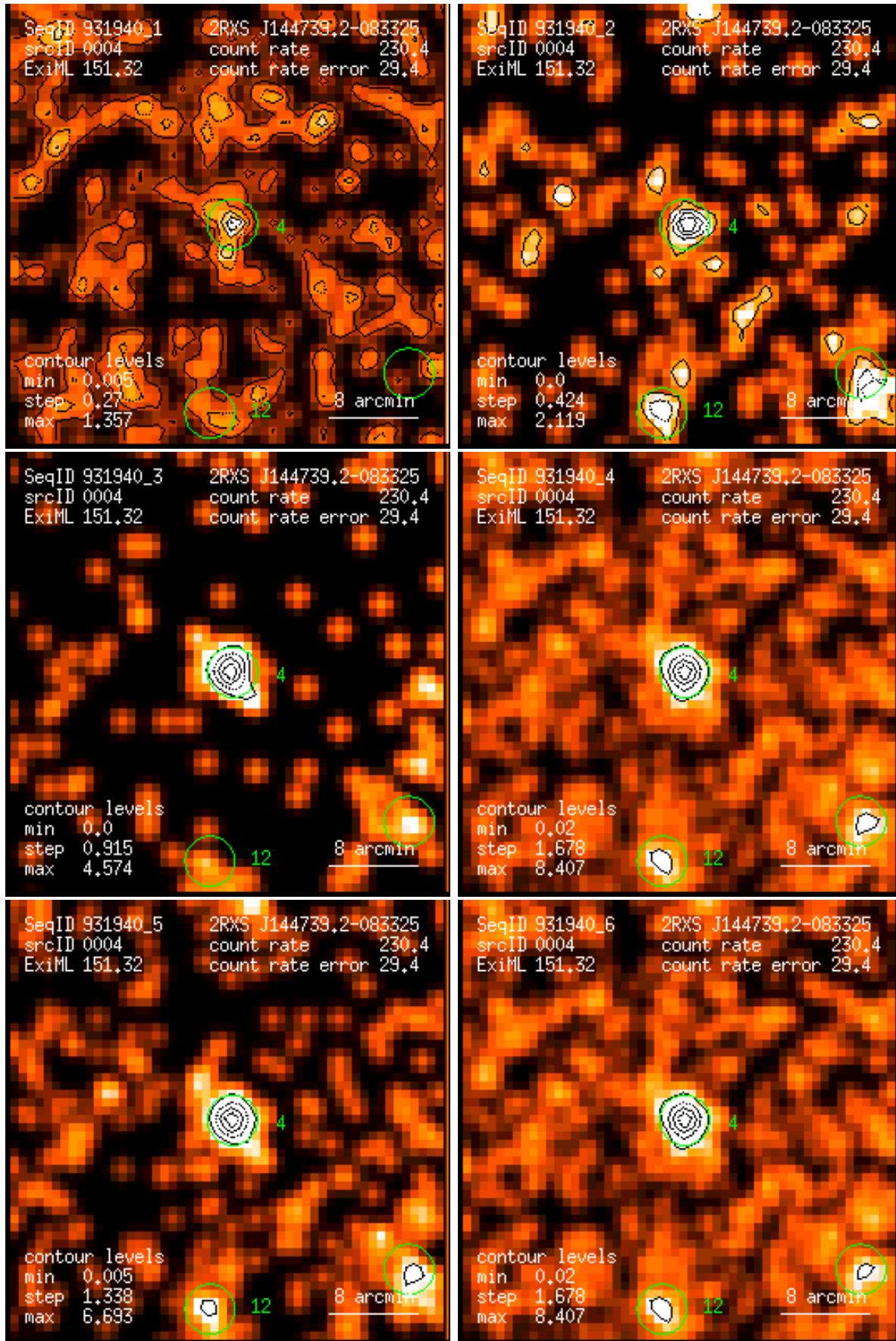
Figure 4: RASS 931940: detection 0004: band rate images, Gaussian filter: (1) PSPC channels 11 – 41, (2) 52 – 90, (3) 91 – 201, (4) 11 – 235, (5) 52 – 201, (6) 11 – 201. Broad band rates in counts/ks. Band rate contour levels in counts/ks/arcmin 2 .
