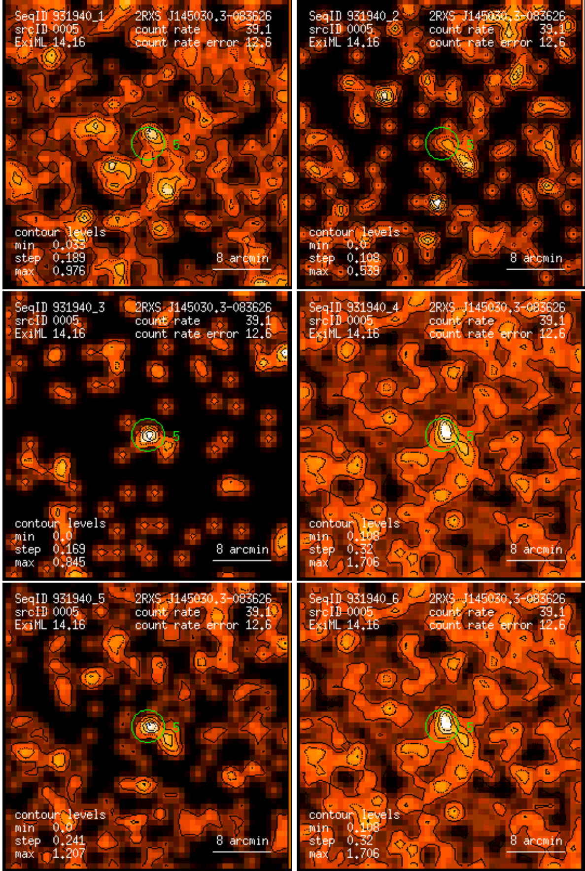
Figure 5: RASS 931940: detection 0005: band rate images, Gaussian filter: (1) PSPC channels 11 – 41, (2) 52 – 90, (3) 91 – 201, (4) 11 – 235, (5) 52 – 201, (6) 11 – 201. Broad band rates in counts/ks. Band rate contour levels in counts/ks/arcmin 2 .
