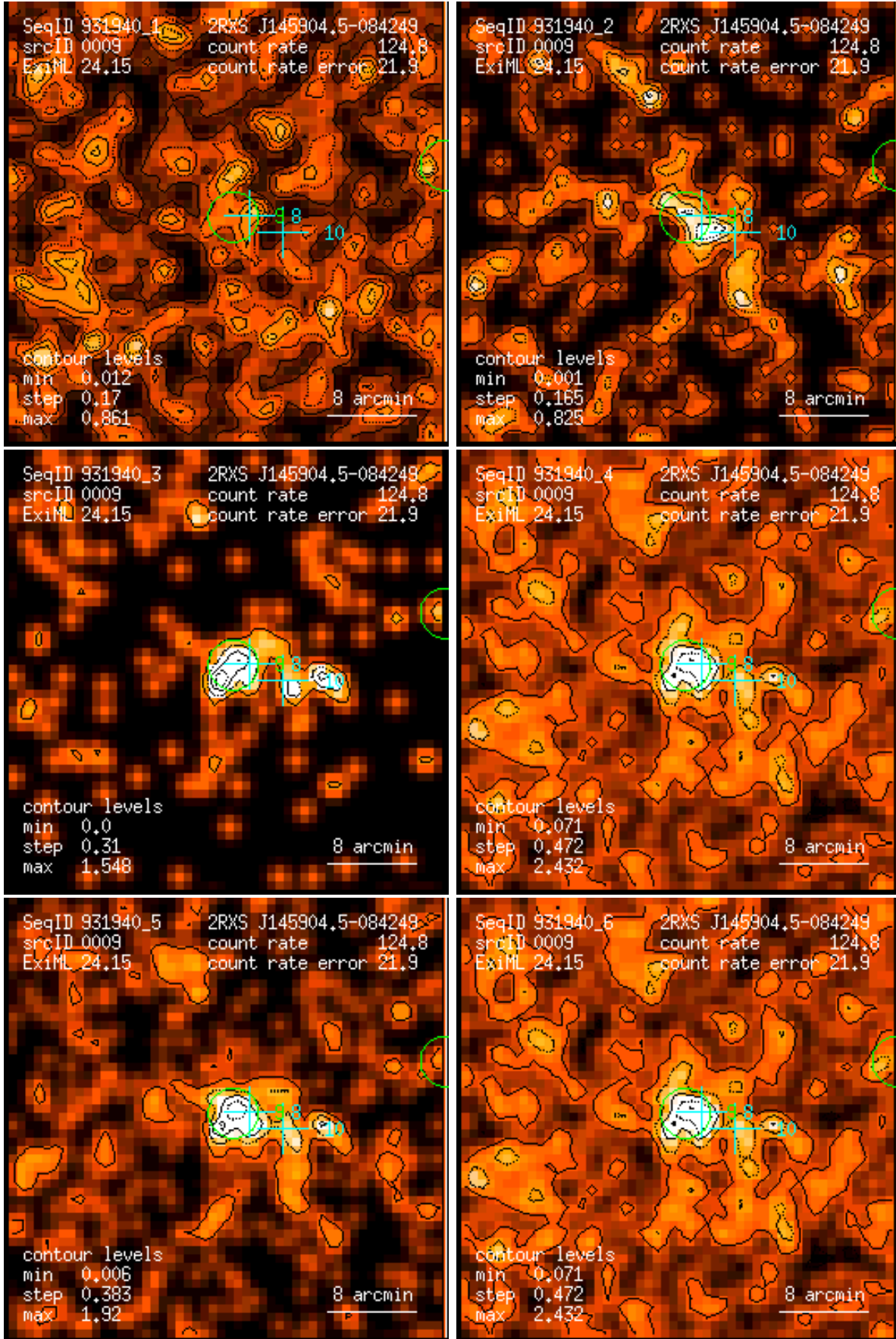
Figure 9: RASS 931940: detection 0009: band rate images, Gaussian filter: (1) PSPC channels 11 – 41, (2) 52 – 90, (3) 91 – 201, (4) 11 – 235, (5) 52 – 201, (6) 11 – 201. Broad band rates in counts/ks. Band rate contour levels in counts/ks/arcmin 2 .
