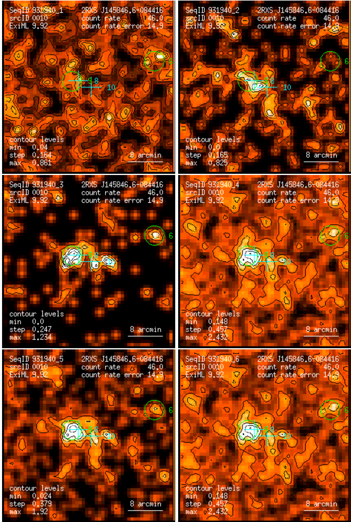
Figure 10: RASS 931940: detection 0010: band rate images, Gaussian filter: (1) PSPC channels 11 – 41, (2) 52 – 90, (3) 91 – 201, (4) 11 – 235, (5) 52 – 201, (6) 11 – 201. Broad band rates in counts/ks. Band rate contour levels in counts/ks/arcmin 2 .
