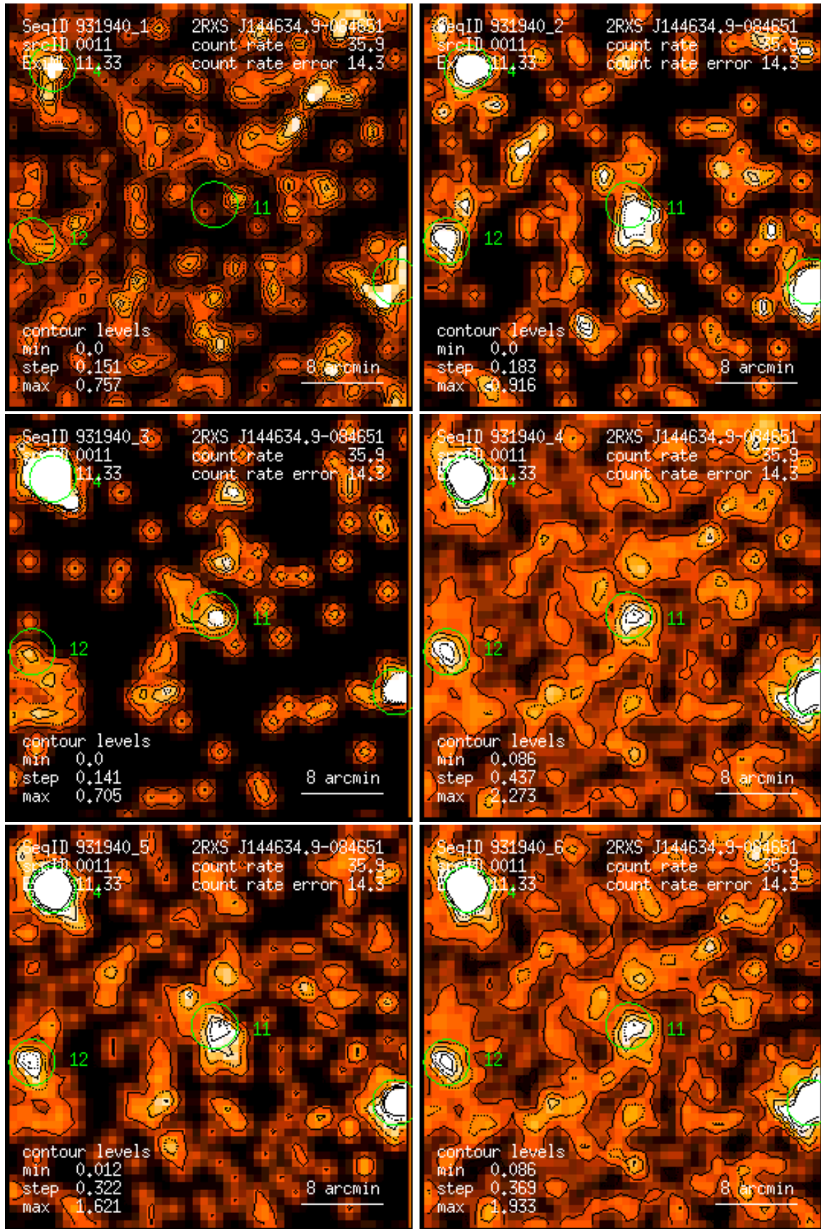
Figure 11: RASS 931940: detection 0011: band rate images, Gaussian filter: (1) PSPC channels 11 – 41, (2) 52 – 90, (3) 91 – 201, (4) 11 – 235, (5) 52 – 201, (6) 11 – 201. Broad band rates in counts/ks. Band rate contour levels in counts/ks/arcmin 2 .
