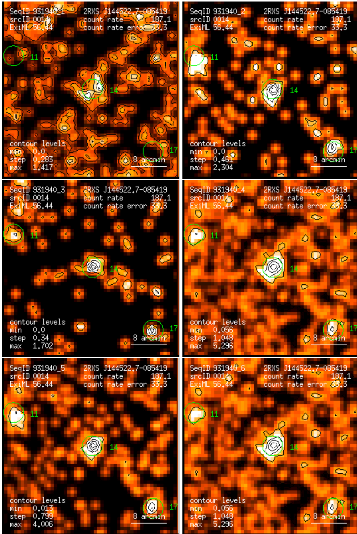
Figure 14: RASS 931940: detection 0014: band rate images, Gaussian filter: (1) PSPC channels 11 – 41, (2) 52 – 90, (3) 91 – 201, (4) 11 – 235, (5) 52 – 201, (6) 11 – 201. Broad band rates in counts/ks. Band rate contour levels in counts/ks/arcmin 2 .
