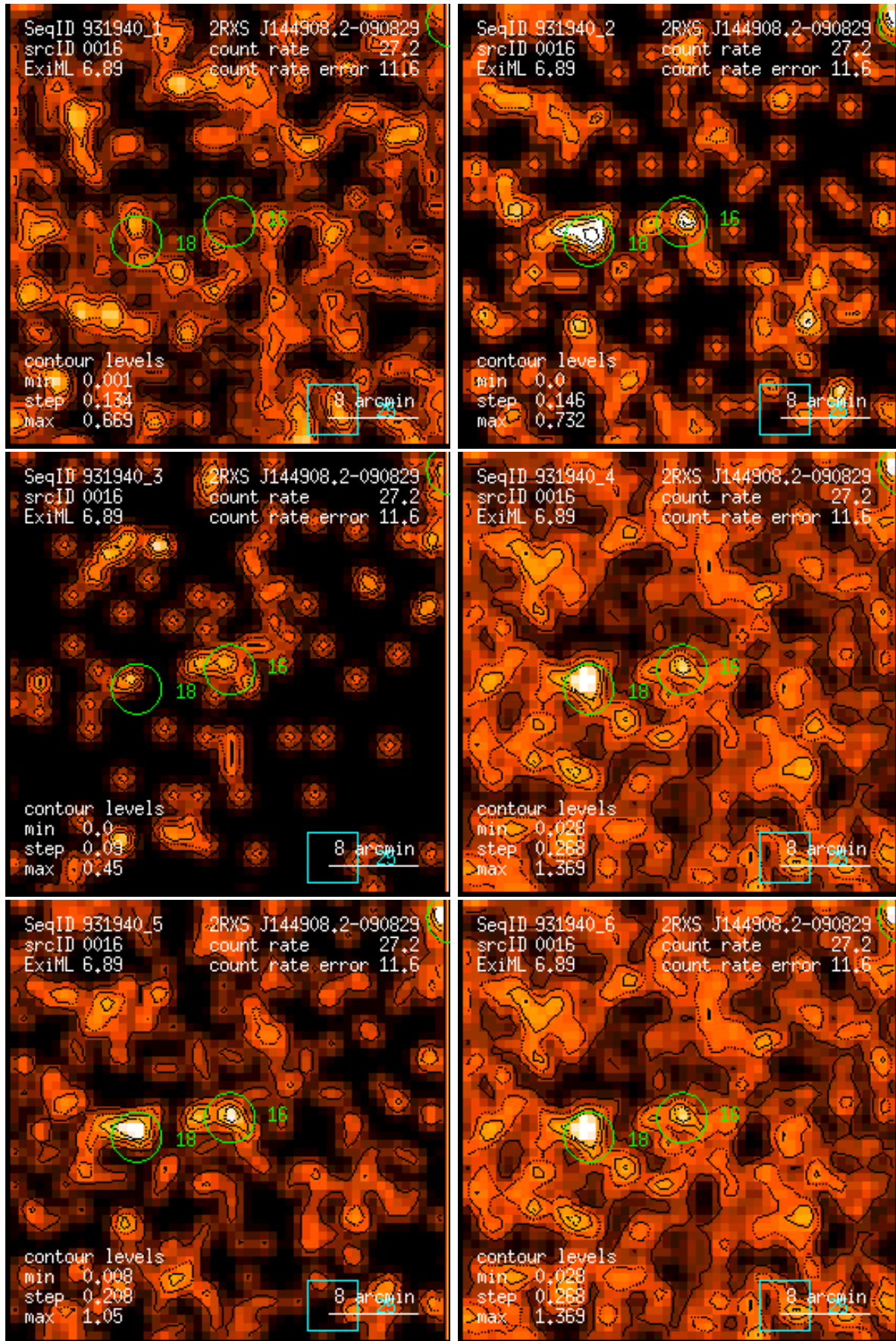
Figure 16: RASS 931940: detection 0016: band rate images, Gaussian filter: (1) PSPC channels 11 – 41, (2) 52 – 90, (3) 91 – 201, (4) 11 – 235, (5) 52 – 201, (6) 11 – 201. Broad band rates in counts/ks. Band rate contour levels in counts/ks/arcmin 2 .
