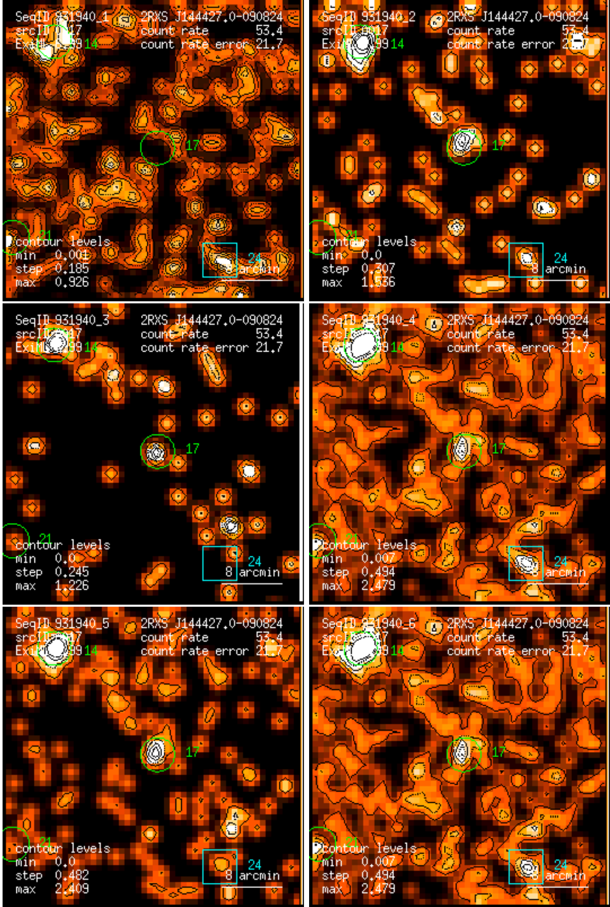
Figure 17: RASS 931940: detection 0017: band rate images, Gaussian filter: (1) PSPC channels 11 – 41, (2) 52 – 90, (3) 91 – 201, (4) 11 – 235, (5) 52 – 201, (6) 11 – 201. Broad band rates in counts/ks. Band rate contour levels in counts/ks/arcmin 2 .
