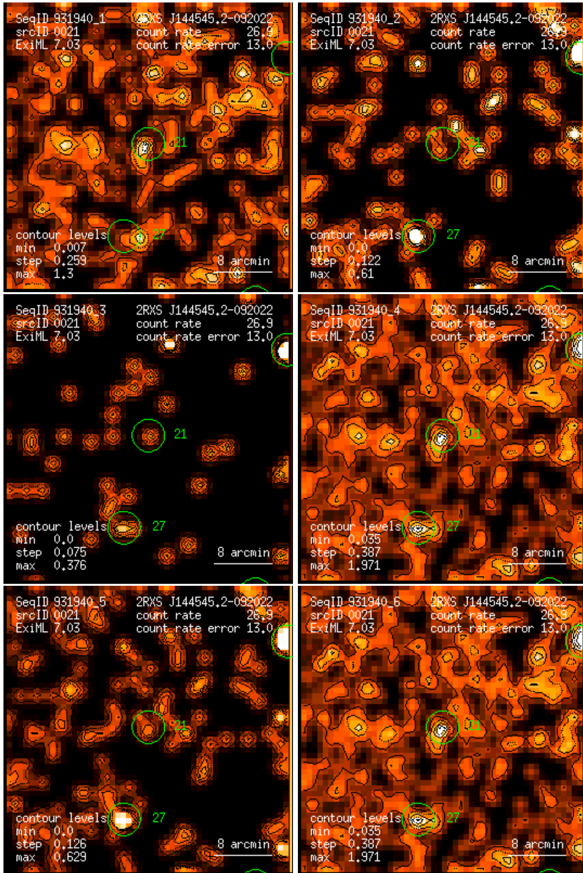
Figure 21: RASS 931940: detection 0021: band rate images, Gaussian filter: (1) PSPC channels 11 – 41, (2) 52 – 90, (3) 91 – 201, (4) 11 – 235, (5) 52 – 201, (6) 11 – 201. Broad band rates in counts/ks. Band rate contour levels in counts/ks/arcmin 2 .
