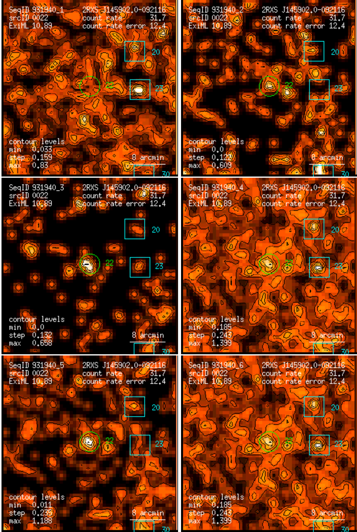
Figure 22: RASS 931940: detection 0022: band rate images, Gaussian filter: (1) PSPC channels 11 – 41, (2) 52 – 90, (3) 91 – 201, (4) 11 – 235, (5) 52 – 201, (6) 11 – 201. Broad band rates in counts/ks. Band rate contour levels in counts/ks/arcmin 2 .
