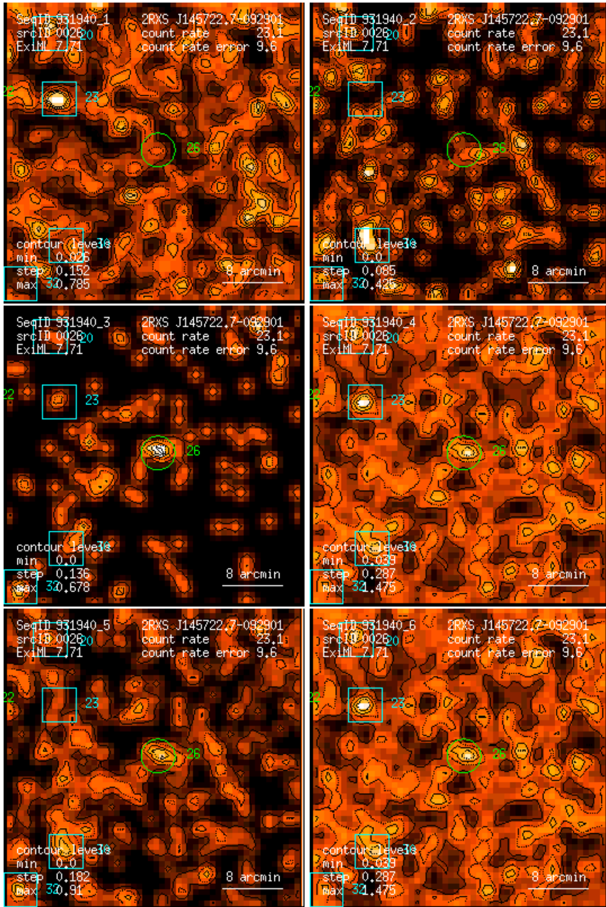
Figure 26: RASS 931940: detection 0026: band rate images, Gaussian filter: (1) PSPC channels 11 – 41, (2) 52 – 90, (3) 91 – 201, (4) 11 – 235, (5) 52 – 201, (6) 11 – 201. Broad band rates in counts/ks. Band rate contour levels in counts/ks/arcmin 2 .
