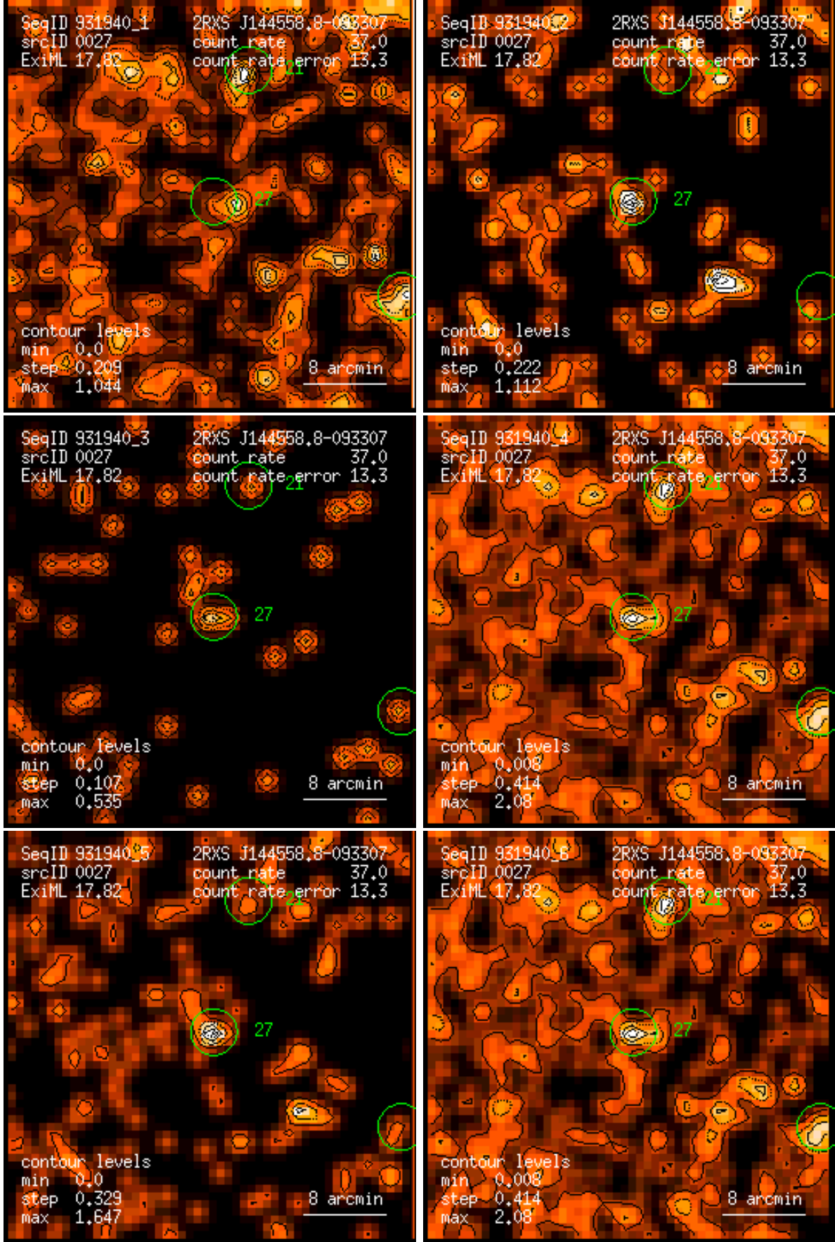
Figure 27: RASS 931940: detection 0027: band rate images, Gaussian filter: (1) PSPC channels 11 – 41, (2) 52 – 90, (3) 91 – 201, (4) 11 – 235, (5) 52 – 201, (6) 11 – 201. Broad band rates in counts/ks. Band rate contour levels in counts/ks/arcmin 2 .
