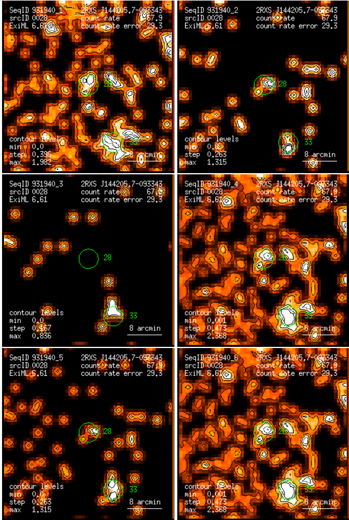
Figure 28: RASS 931940: detection 0028: band rate images, Gaussian filter: (1) PSPC channels 11 – 41, (2) 52 – 90, (3) 91 – 201, (4) 11 – 235, (5) 52 – 201, (6) 11 – 201. Broad band rates in counts/ks. Band rate contour levels in counts/ks/arcmin 2 .
