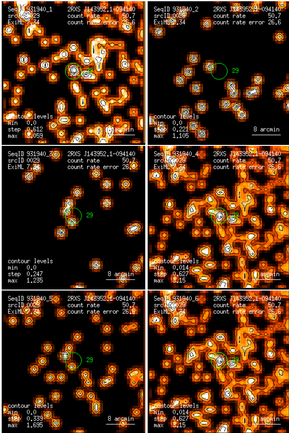
Figure 29: RASS 931940: detection 0029: band rate images, Gaussian filter: (1) PSPC channels 11 – 41, (2) 52 – 90, (3) 91 – 201, (4) 11 – 235, (5) 52 – 201, (6) 11 – 201. Broad band rates in counts/ks. Band rate contour levels in counts/ks/arcmin 2 .
