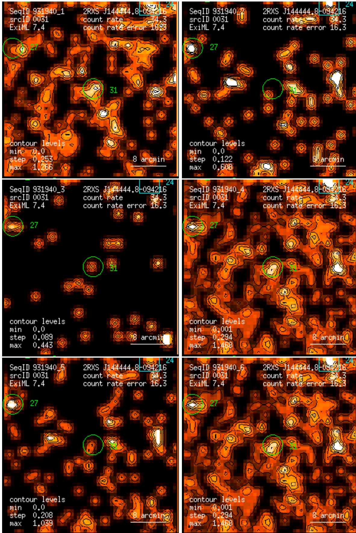
Figure 31: RASS 931940: detection 0031: band rate images, Gaussian filter: (1) PSPC channels 11 – 41, (2) 52 – 90, (3) 91 – 201, (4) 11 – 235, (5) 52 – 201, (6) 11 – 201. Broad band rates in counts/ks. Band rate contour levels in counts/ks/arcmin 2 .
