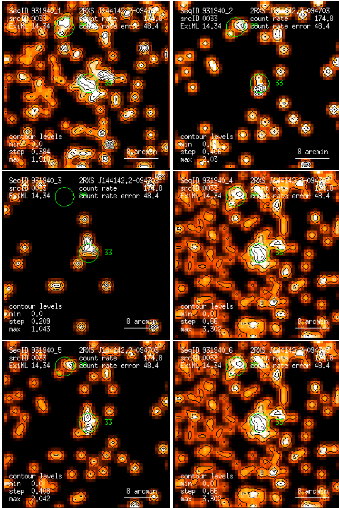
Figure 33: RASS 931940: detection 0033: band rate images, Gaussian filter: (1) PSPC channels 11 – 41, (2) 52 – 90, (3) 91 – 201, (4) 11 – 235, (5) 52 – 201, (6) 11 – 201. Broad band rates in counts/ks. Band rate contour levels in counts/ks/arcmin 2 .
