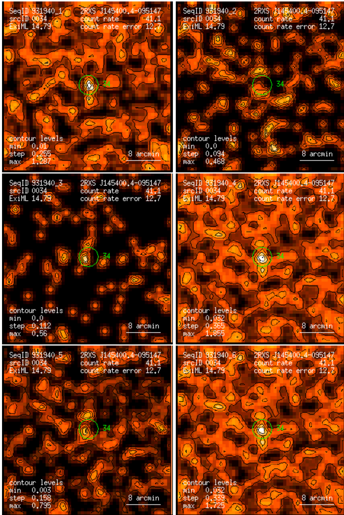
Figure 34: RASS 931940: detection 0034: band rate images, Gaussian filter: (1) PSPC channels 11 – 41, (2) 52 – 90, (3) 91 – 201, (4) 11 – 235, (5) 52 – 201, (6) 11 – 201. Broad band rates in counts/ks. Band rate contour levels in counts/ks/arcmin 2 .
