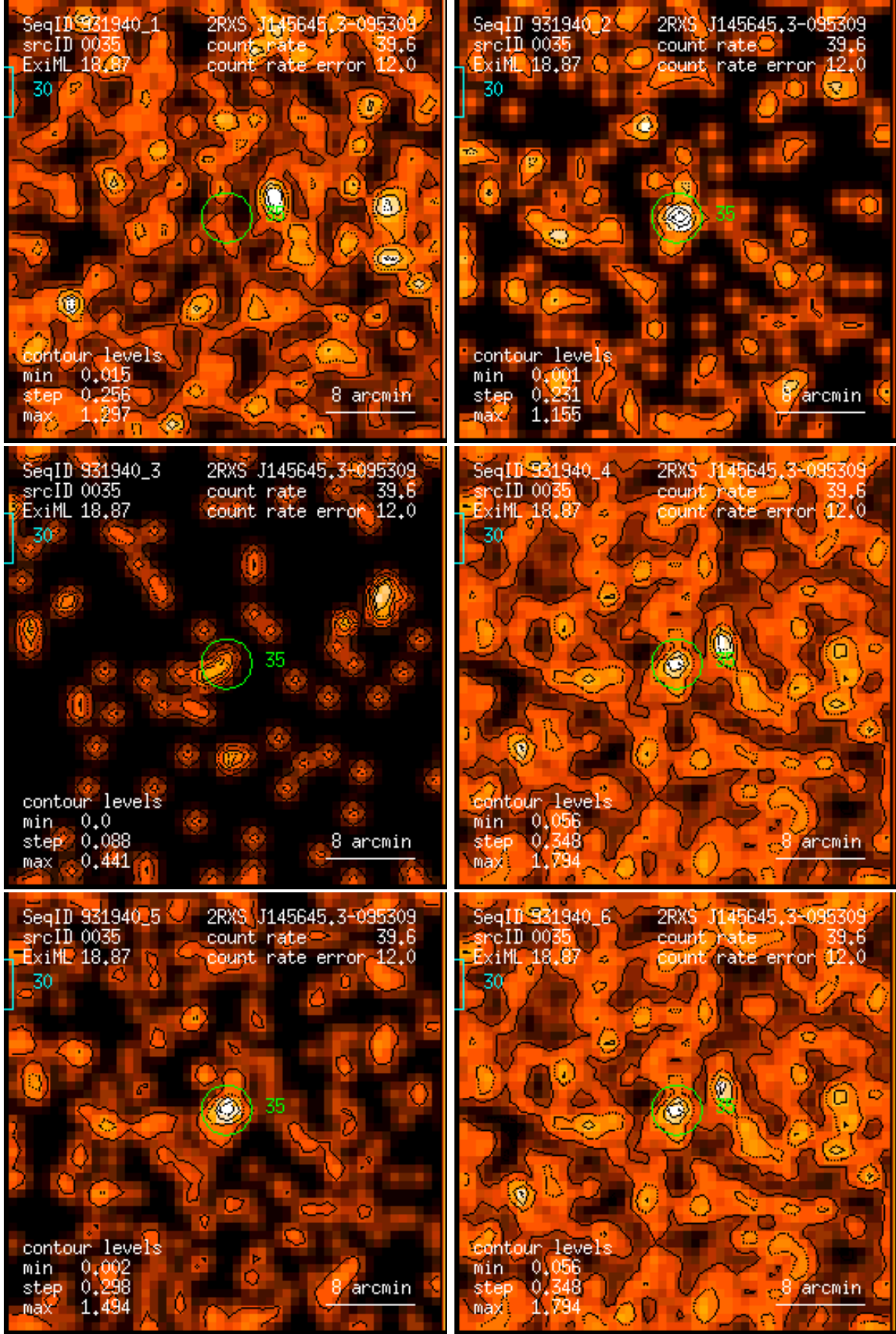
Figure 35: RASS 931940: detection 0035: band rate images, Gaussian filter: (1) PSPC channels 11 – 41, (2) 52 – 90, (3) 91 – 201, (4) 11 – 235, (5) 52 – 201, (6) 11 – 201. Broad band rates in counts/ks. Band rate contour levels in counts/ks/arcmin 2 .
