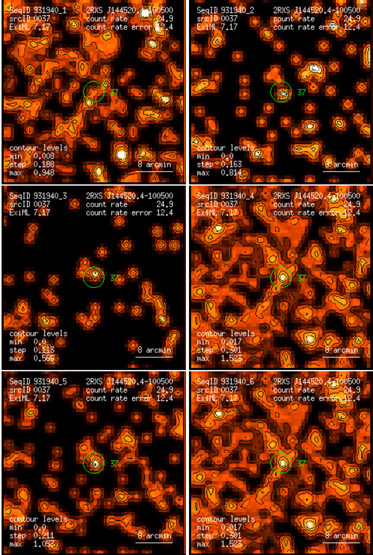
Figure 37: RASS 931940: detection 0037: band rate images, Gaussian filter: (1) PSPC channels 11 – 41, (2) 52 – 90, (3) 91 – 201, (4) 11 – 235, (5) 52 – 201, (6) 11 – 201. Broad band rates in counts/ks. Band rate contour levels in counts/ks/arcmin 2 .
