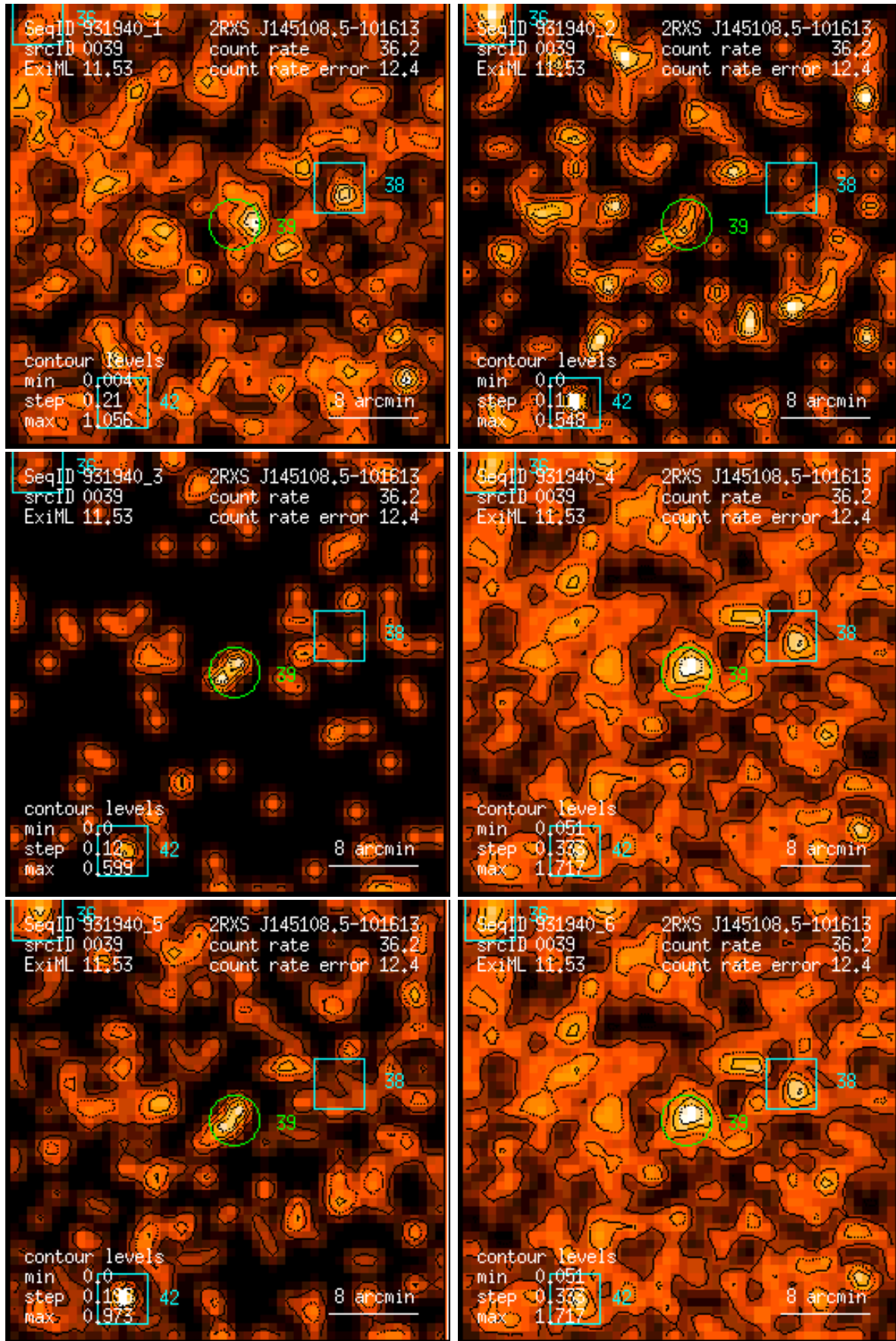
Figure 39: RASS 931940: detection 0039: band rate images, Gaussian filter: (1) PSPC channels 11 – 41, (2) 52 – 90, (3) 91 – 201, (4) 11 – 235, (5) 52 – 201, (6) 11 – 201. Broad band rates in counts/ks. Band rate contour levels in counts/ks/arcmin 2 .
