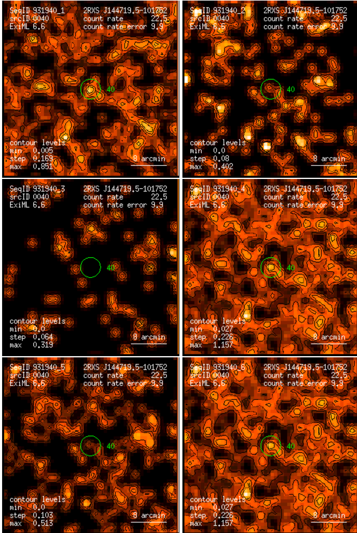
Figure 40: RASS 931940: detection 0040: band rate images, Gaussian filter: (1) PSPC channels 11 – 41, (2) 52 – 90, (3) 91 – 201, (4) 11 – 235, (5) 52 – 201, (6) 11 – 201. Broad band rates in counts/ks. Band rate contour levels in counts/ks/arcmin 2 .
