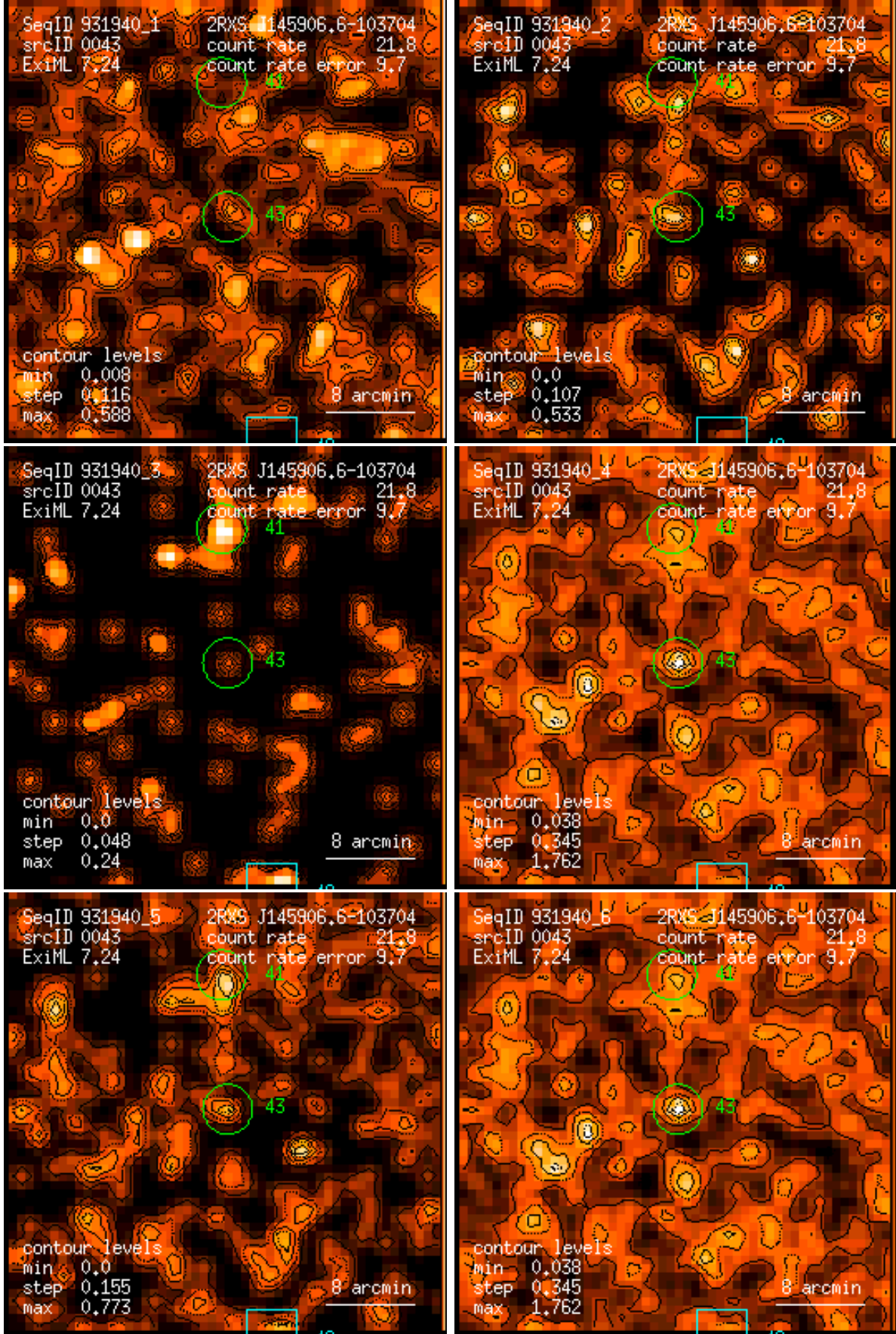
Figure 43: RASS 931940: detection 0043: band rate images, Gaussian filter: (1) PSPC channels 11 – 41, (2) 52 – 90, (3) 91 – 201, (4) 11 – 235, (5) 52 – 201, (6) 11 – 201. Broad band rates in counts/ks. Band rate contour levels in counts/ks/arcmin 2 .
