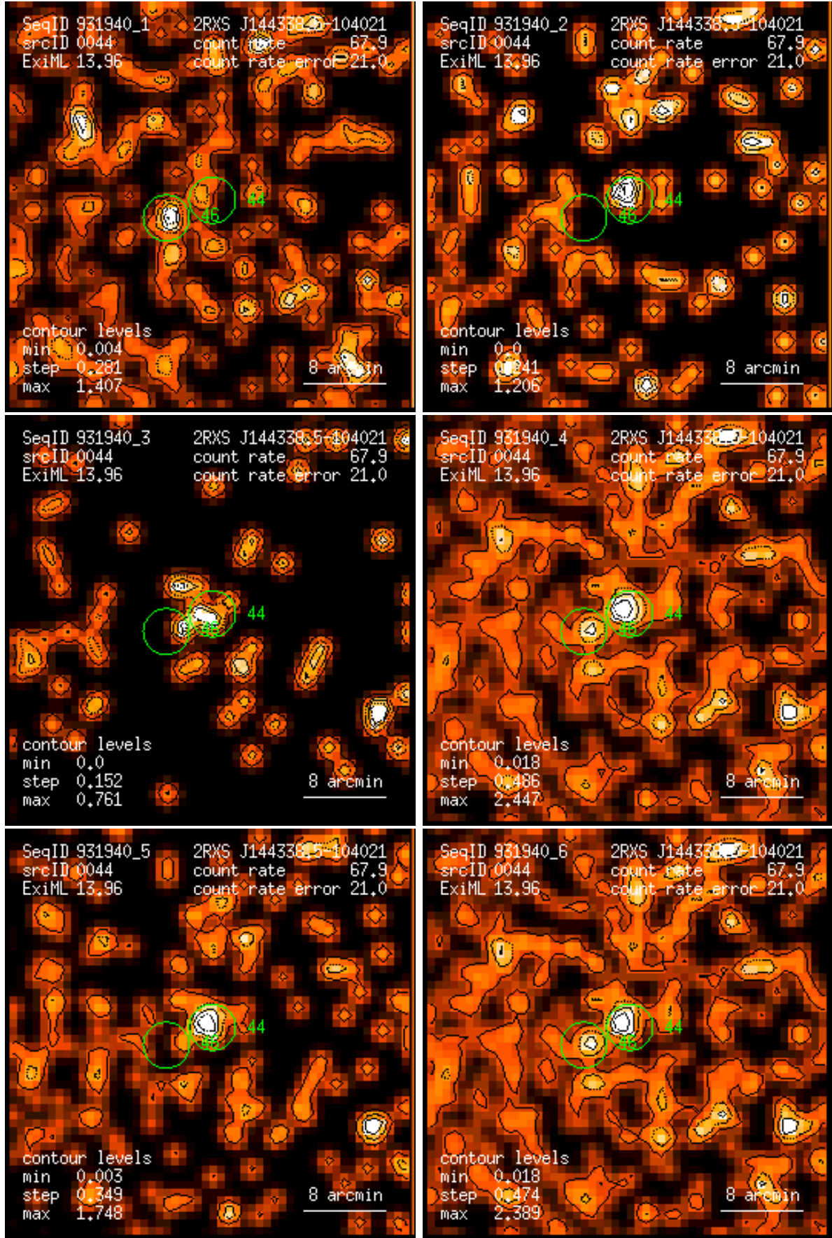
Figure 44: RASS 931940: detection 0044: band rate images, Gaussian filter: (1) PSPC channels 11 – 41, (2) 52 – 90, (3) 91 – 201, (4) 11 – 235, (5) 52 – 201, (6) 11 – 201. Broad band rates in counts/ks. Band rate contour levels in counts/ks/arcmin 2 .
