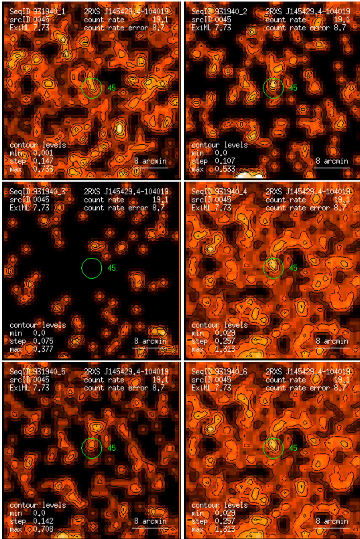
Figure 45: RASS 931940: detection 0045: band rate images, Gaussian filter: (1) PSPC channels 11 – 41, (2) 52 – 90, (3) 91 – 201, (4) 11 – 235, (5) 52 – 201, (6) 11 – 201. Broad band rates in counts/ks. Band rate contour levels in counts/ks/arcmin 2 .
