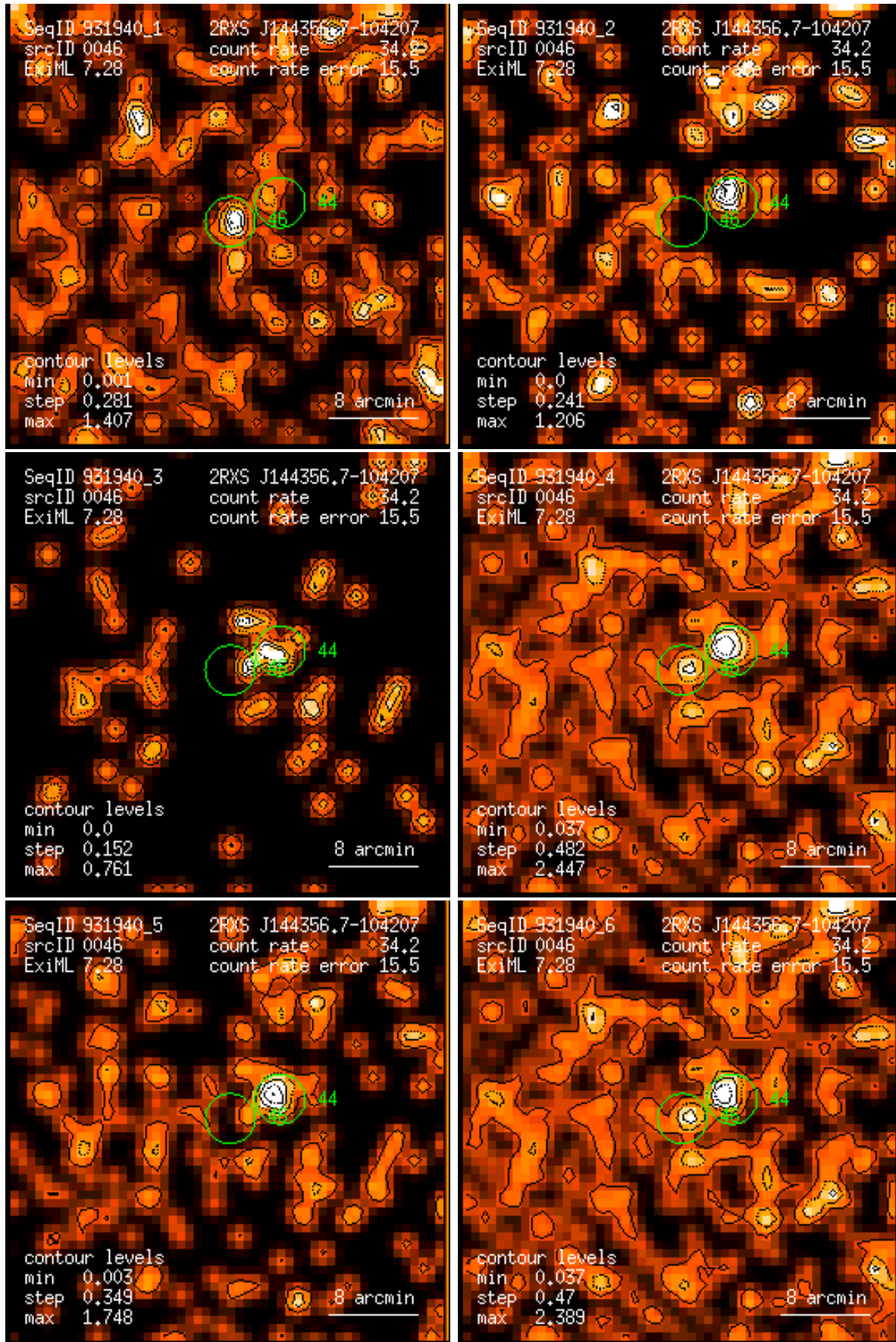
Figure 46: RASS 931940: detection 0046: band rate images, Gaussian filter: (1) PSPC channels 11 – 41, (2) 52 – 90, (3) 91 – 201, (4) 11 – 235, (5) 52 – 201, (6) 11 – 201. Broad band rates in counts/ks. Band rate contour levels in counts/ks/arcmin 2 .
