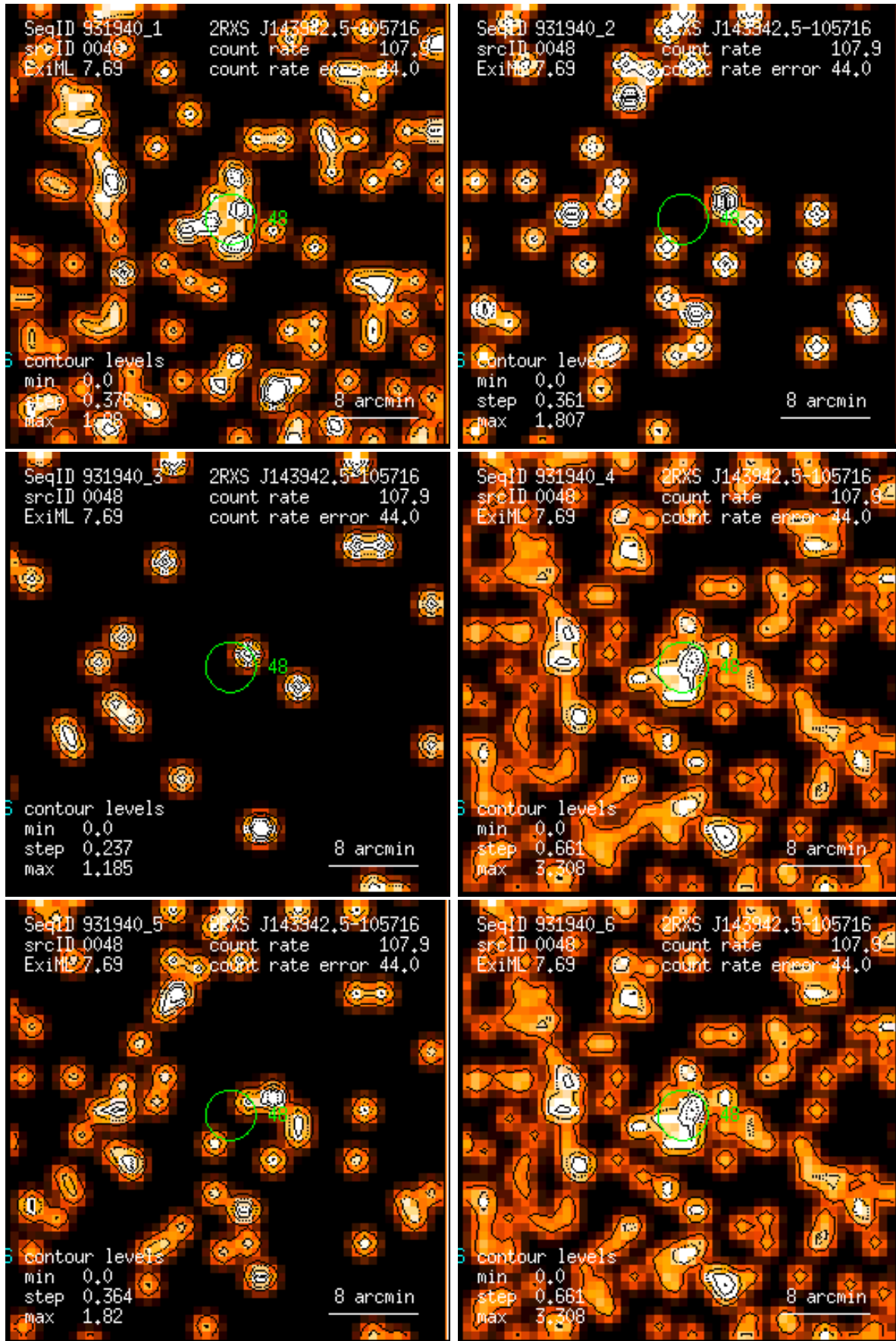
Figure 48: RASS 931940: detection 0048: band rate images, Gaussian filter: (1) PSPC channels 11 – 41, (2) 52 – 90, (3) 91 – 201, (4) 11 – 235, (5) 52 – 201, (6) 11 – 201. Broad band rates in counts/ks. Band rate contour levels in counts/ks/arcmin 2 .
