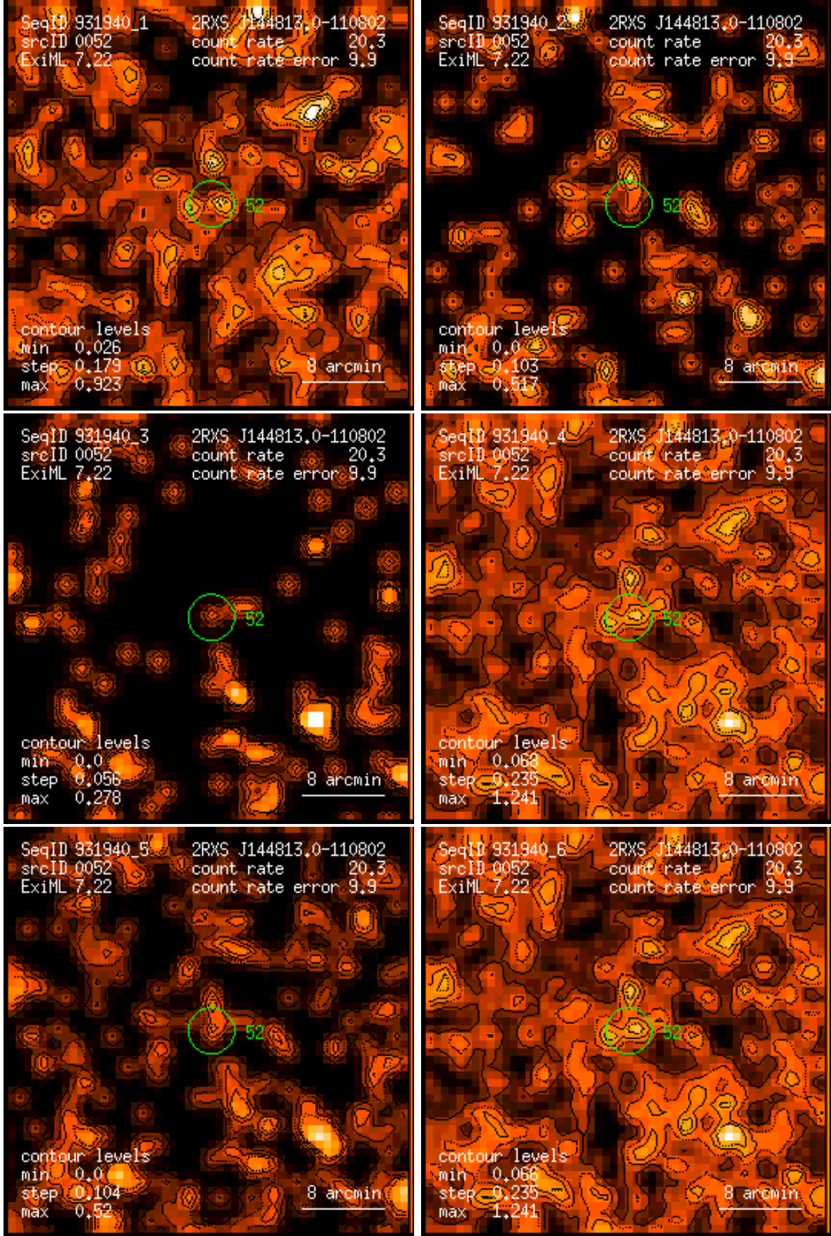
Figure 52: RASS 931940: detection 0052: band rate images, Gaussian filter: (1) PSPP channels 11 – 41, (2) 52 – 90, (3) 91 – 201, (4) 11 – 235, (5) 52 – 201, (6) 11 – 201. Broad band rates in counts/ks. Band rate contour levels in counts/ks/arcmin 2 .
