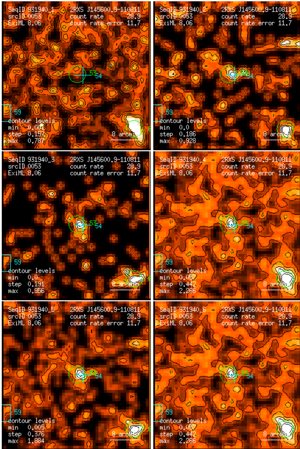
Figure 53: RASS 931940: detection 0053: band rate images, Gaussian filter: (1) PSPC channels 11 – 41, (2) 52 – 90, (3) 91 – 201, (4) 11 – 235, (5) 52 – 201, (6) 11 – 201. Broad band rates in counts/ks. Band rate contour levels in counts/ks/arcmin 2 .
