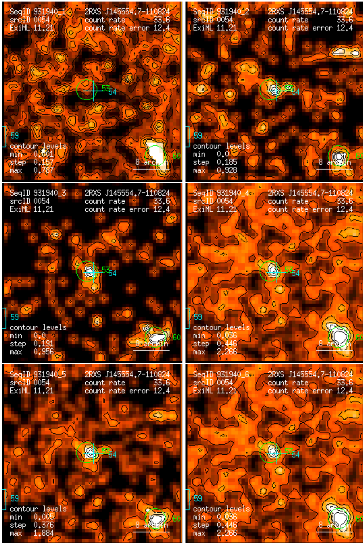
Figure 54: RASS 931940: detection 0054: band rate images, Gaussian filter: (1) PSPC channels 11 – 41, (2) 52 – 90, (3) 91 – 201, (4) 11 – 235, (5) 52 – 201, (6) 11 – 201. Broad band rates in counts/ks. Band rate contour levels in counts/ks/arcmin 2 .
