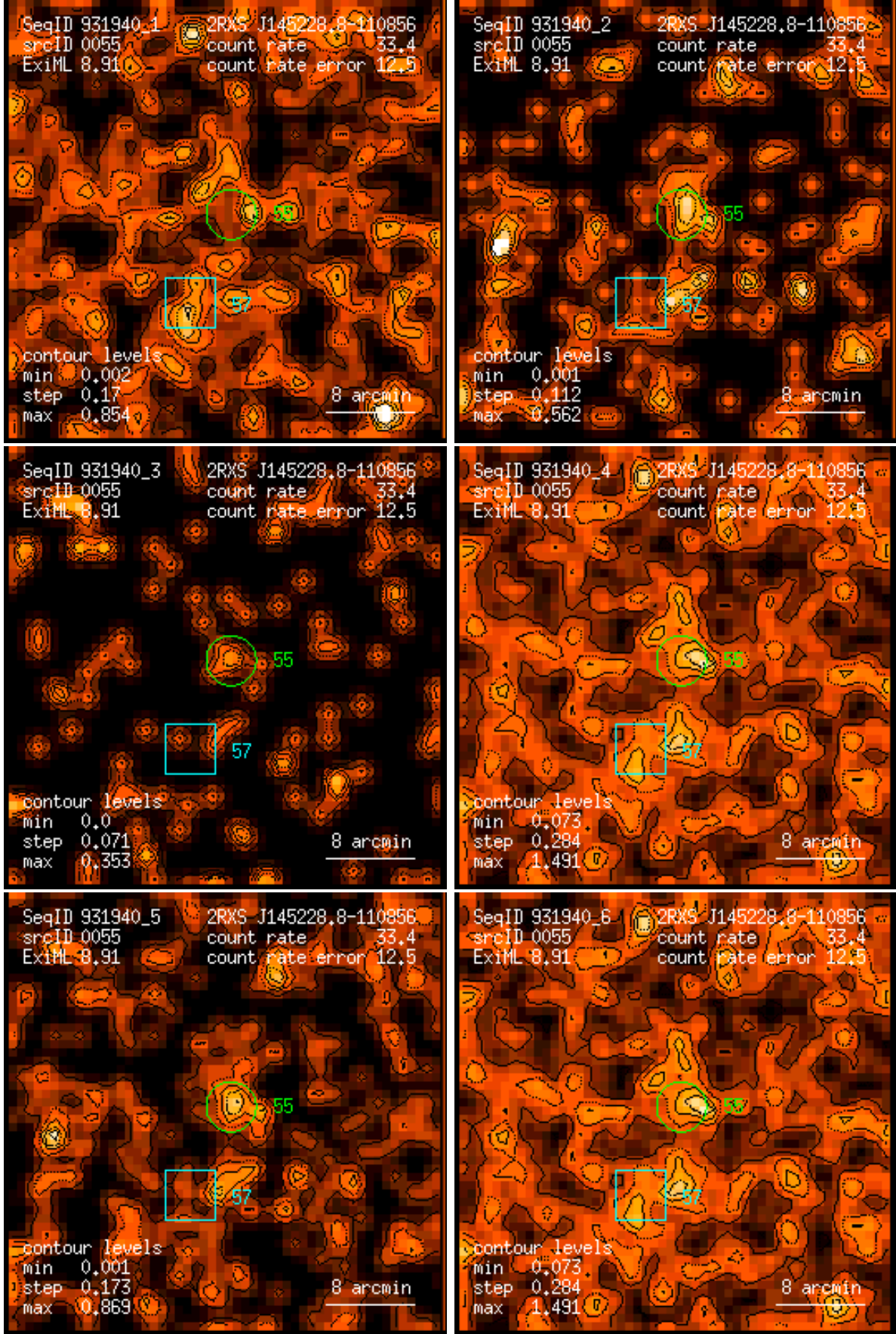
Figure 55: RASS 931940: detection 0055: band rate images, Gaussian filter: (1) PSPC channels 11 – 41, (2) 52 – 90, (3) 91 – 201, (4) 11 – 235, (5) 52 – 201, (6) 11 – 201. Broad band rates in counts/ks. Band rate contour levels in counts/ks/arcmin 2 .
